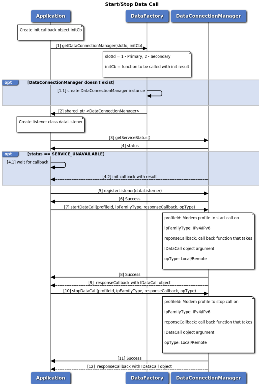
Figure 3-53 Start/Stop data call call flow
