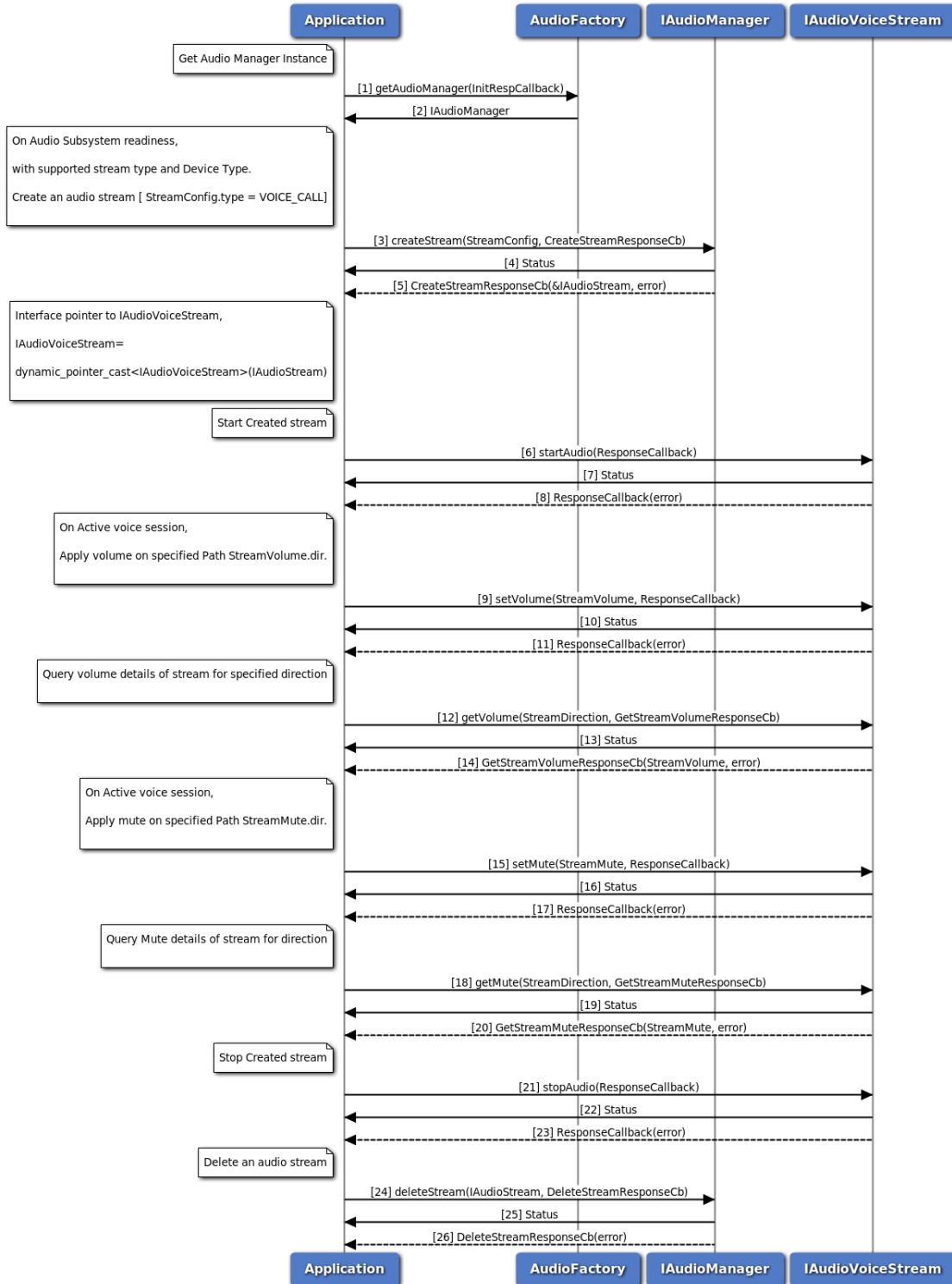
Figure 3-101 Audio Voice Call Volume/Mute control call flow
