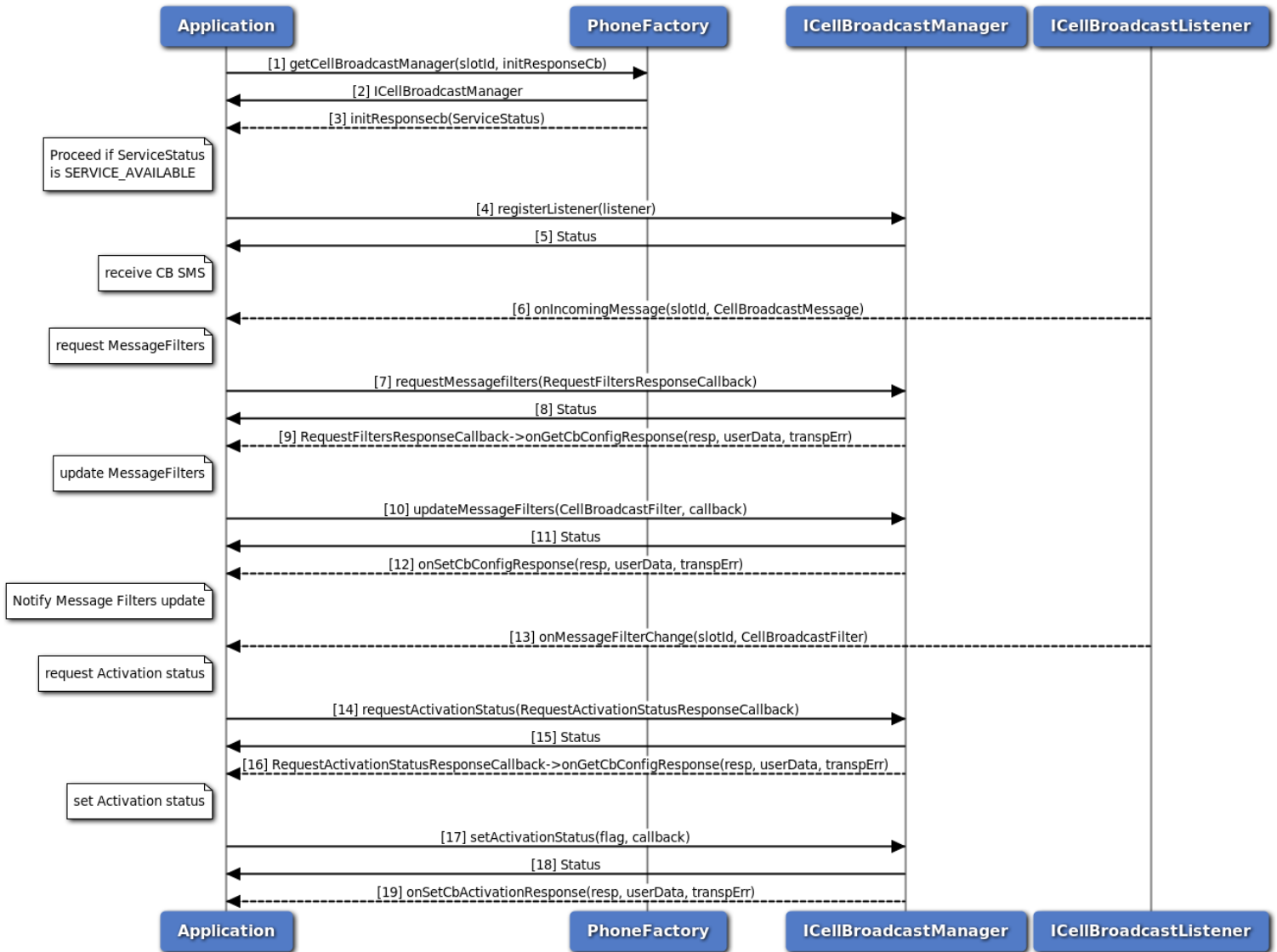
Figure 3-10 CellBroadcast call flow
