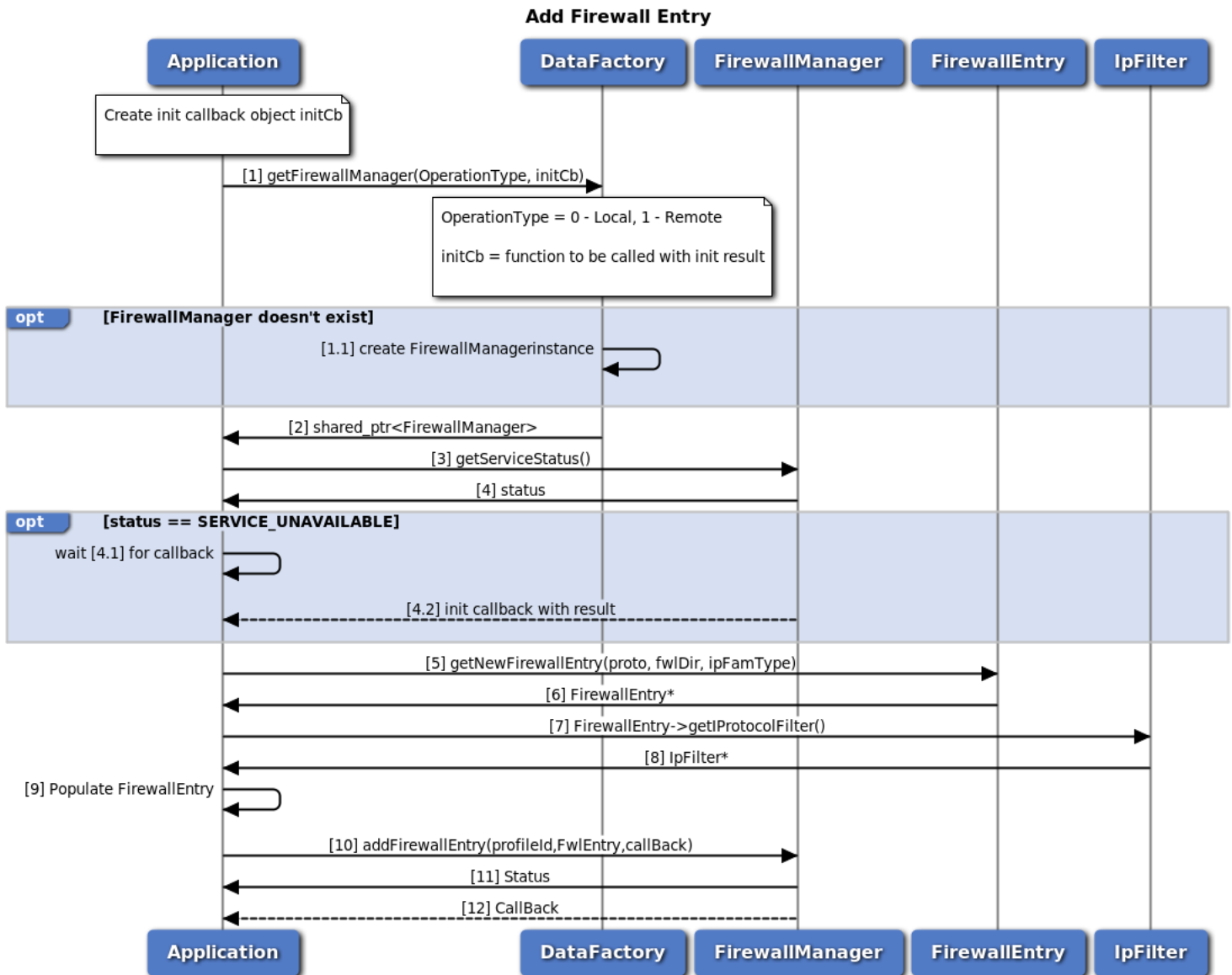
Figure 3-68 Add Firewall entry in data Firewall manager call flow
