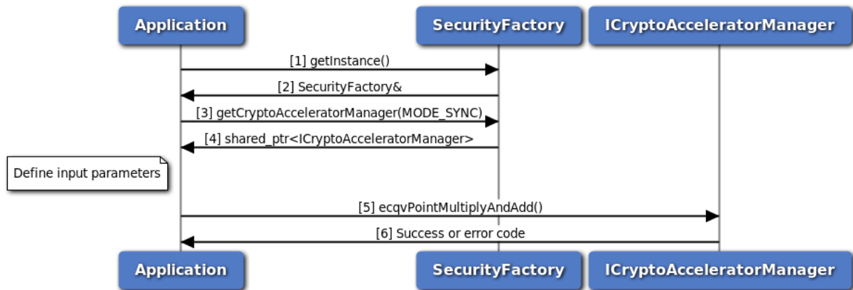
Figure 3-144 Call flow for ECQV calculation synchronous mode
