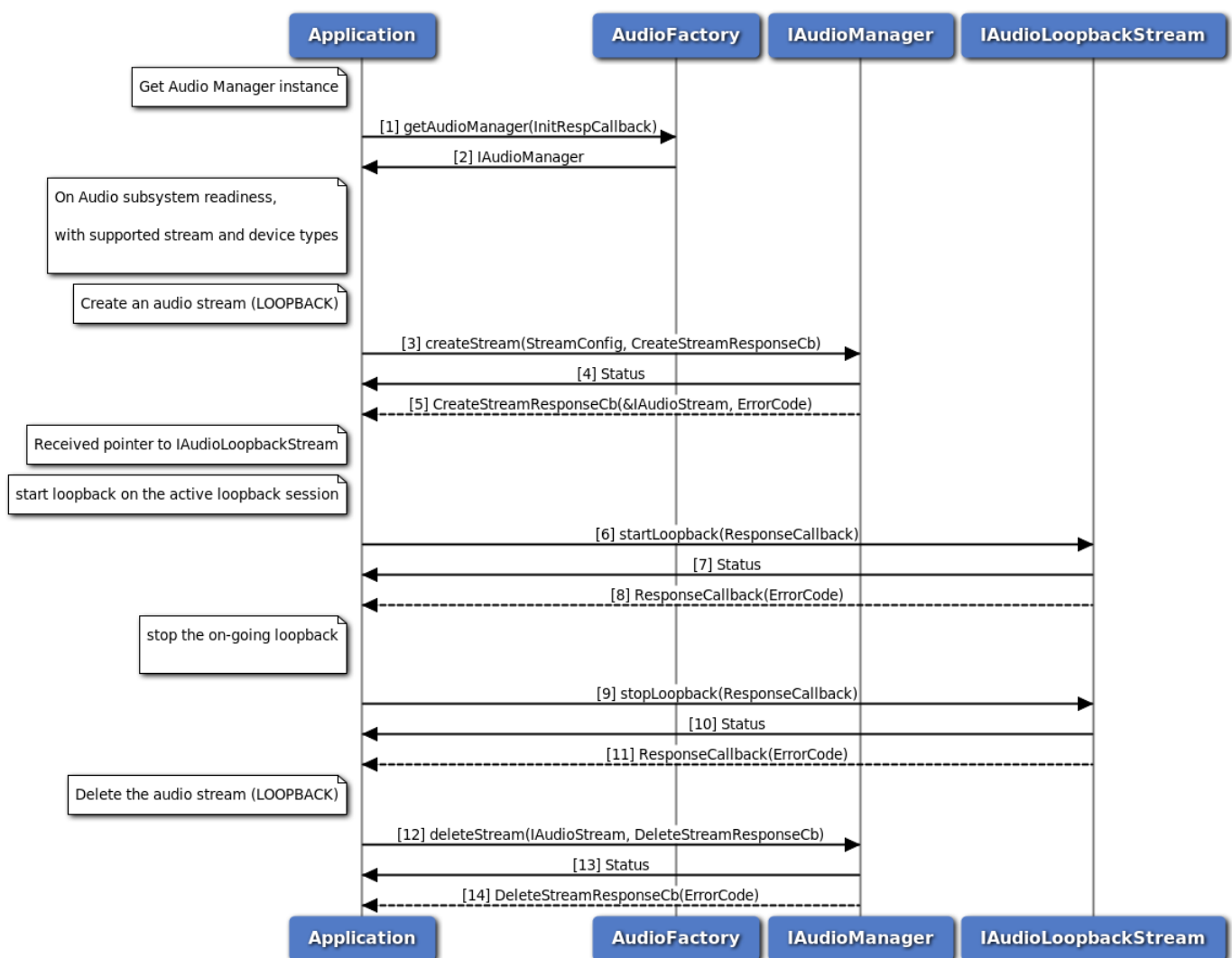
Figure 3-112 Call flow to start/stop loopback between source and sink devices
