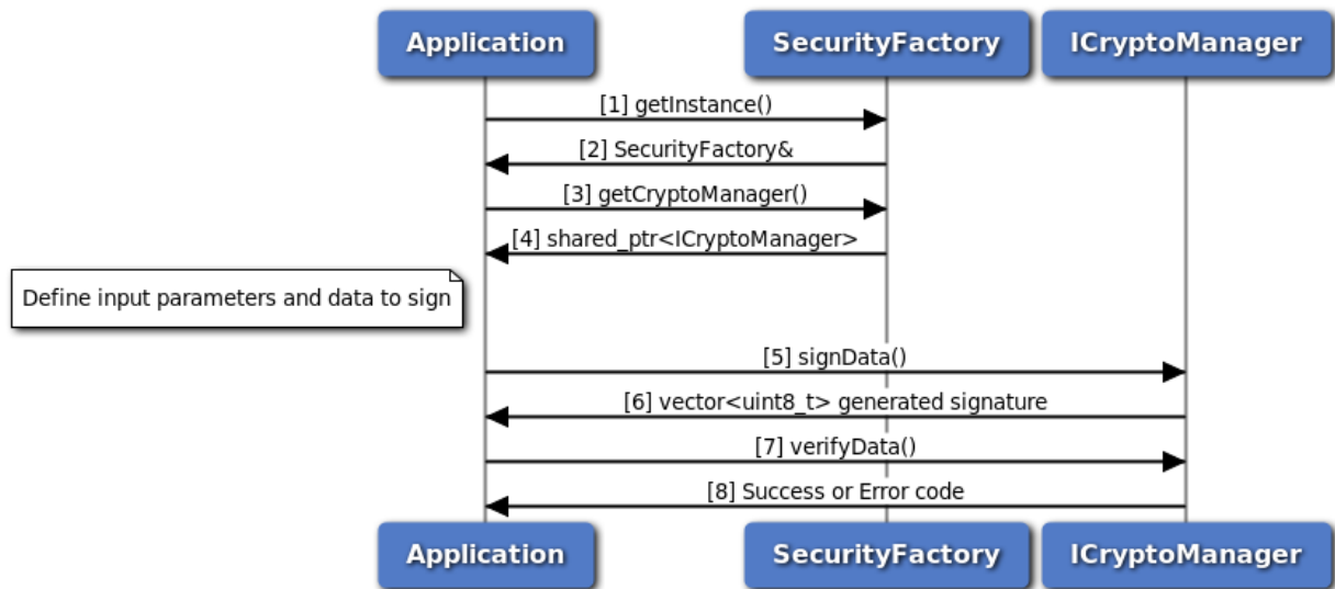
Figure 3-139 Call flow to sign and verify data
