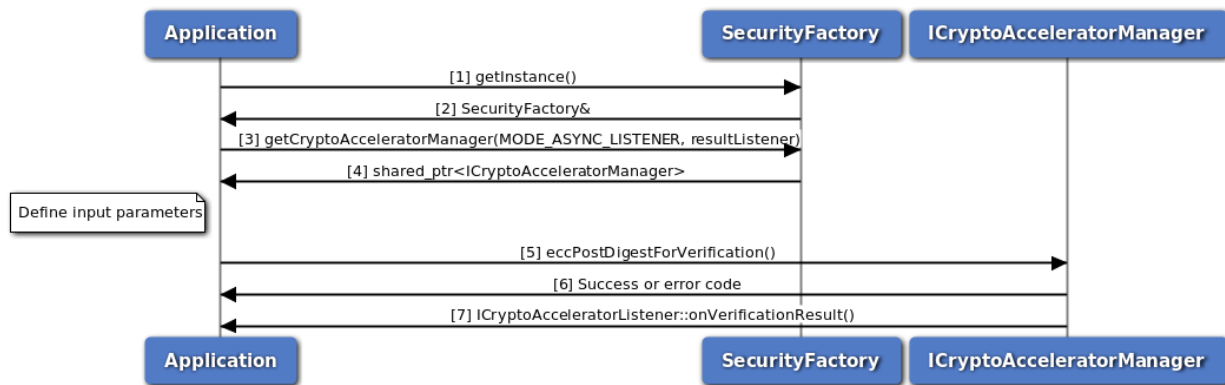
Figure 3-143 Call flow for signature verification asynchronous listener mode
