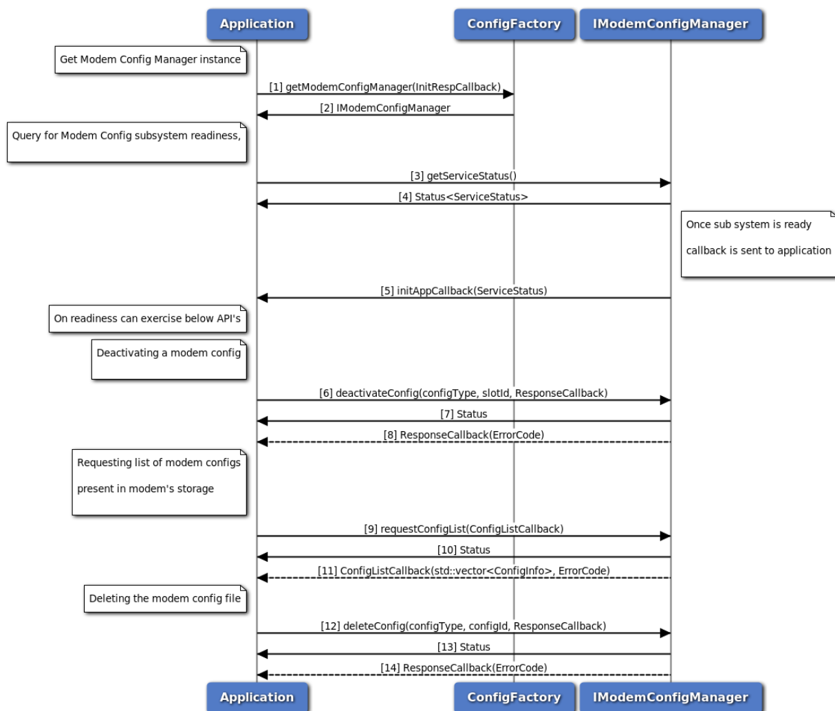
Figure 3-126 Modem Config deactivate and delete Call Flow
