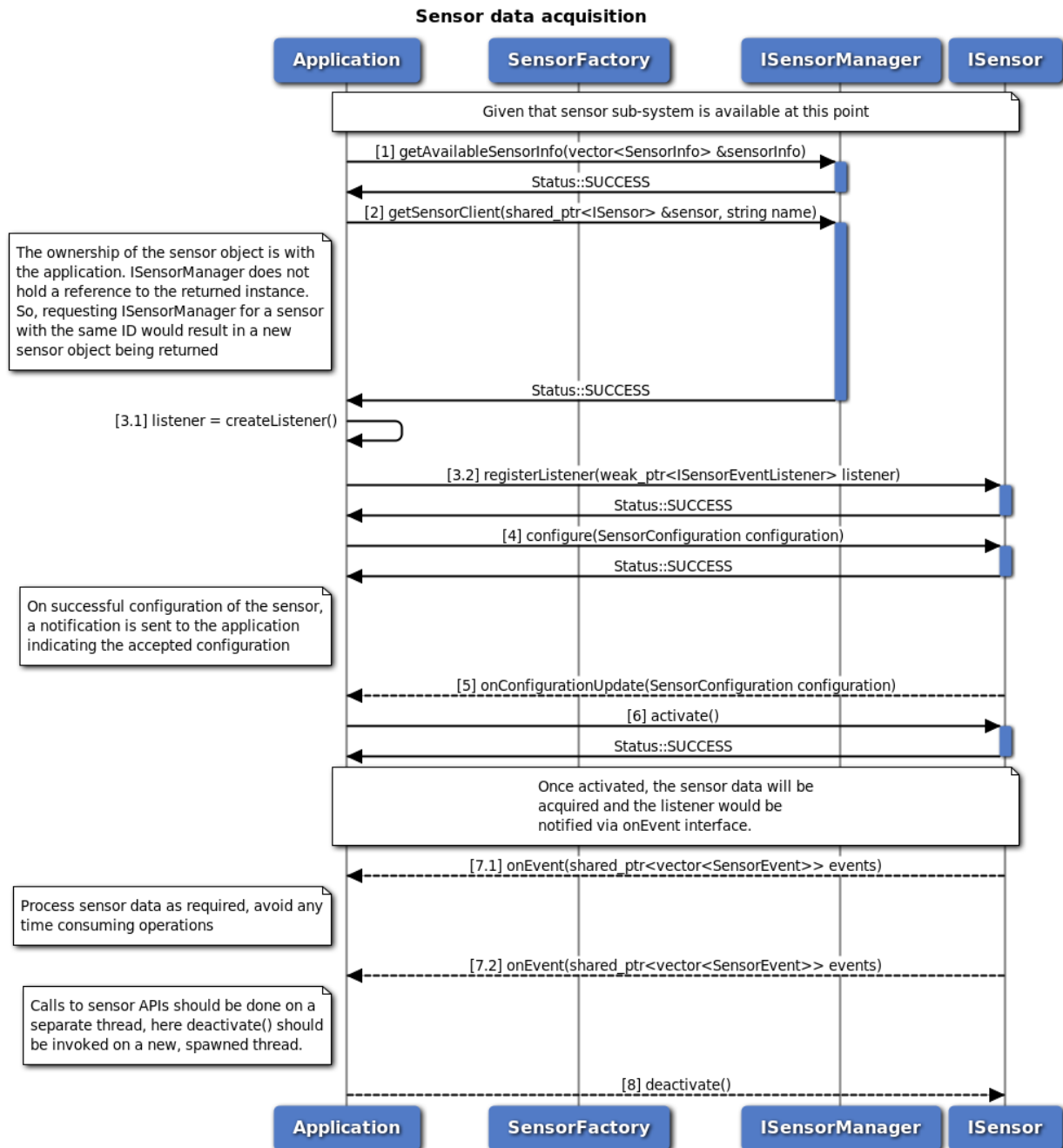
Figure 3-129 Sensor data acquisition call flow
