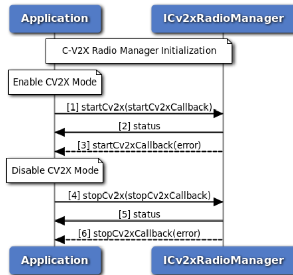
Figure 3-81 Start/Stop C-V2X Mode Call Flow - C++ Version
