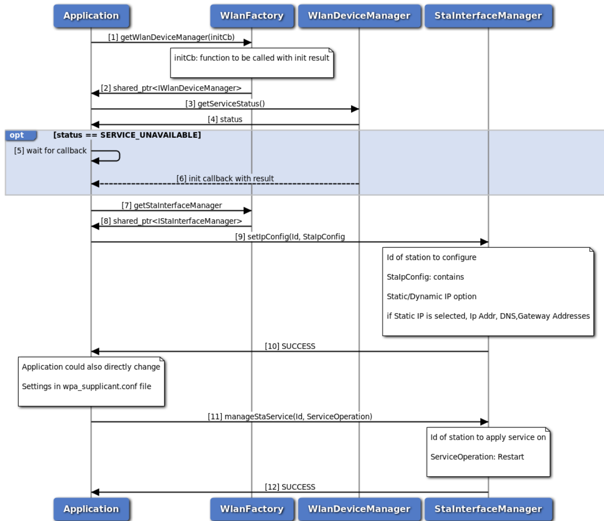
Figure 3-150 Modify WLAN Station Configuration Call Flow
