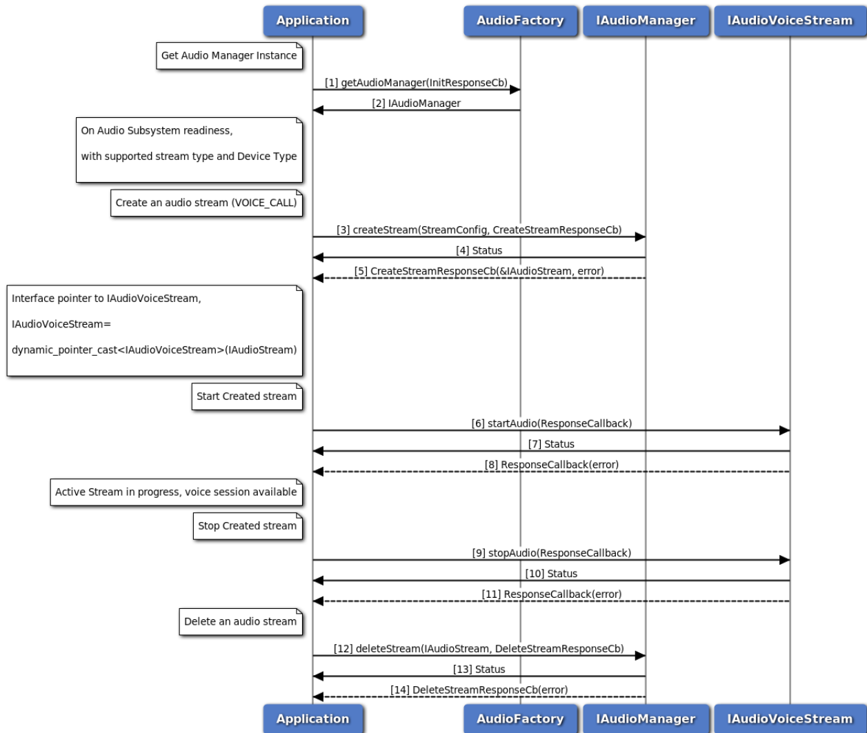
Figure 3-104 Audio Voice Call Start/Stop call flow
