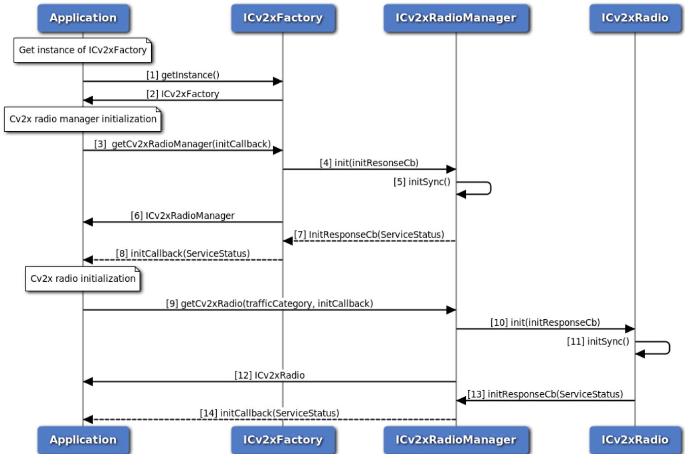
Figure 3-85 C-V2X Radio Initialization Call Flow - C++ Version
