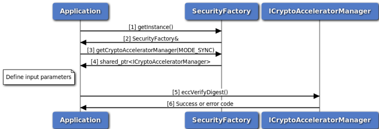
Figure 3-141 Call flow for signature verification synchronous mode
