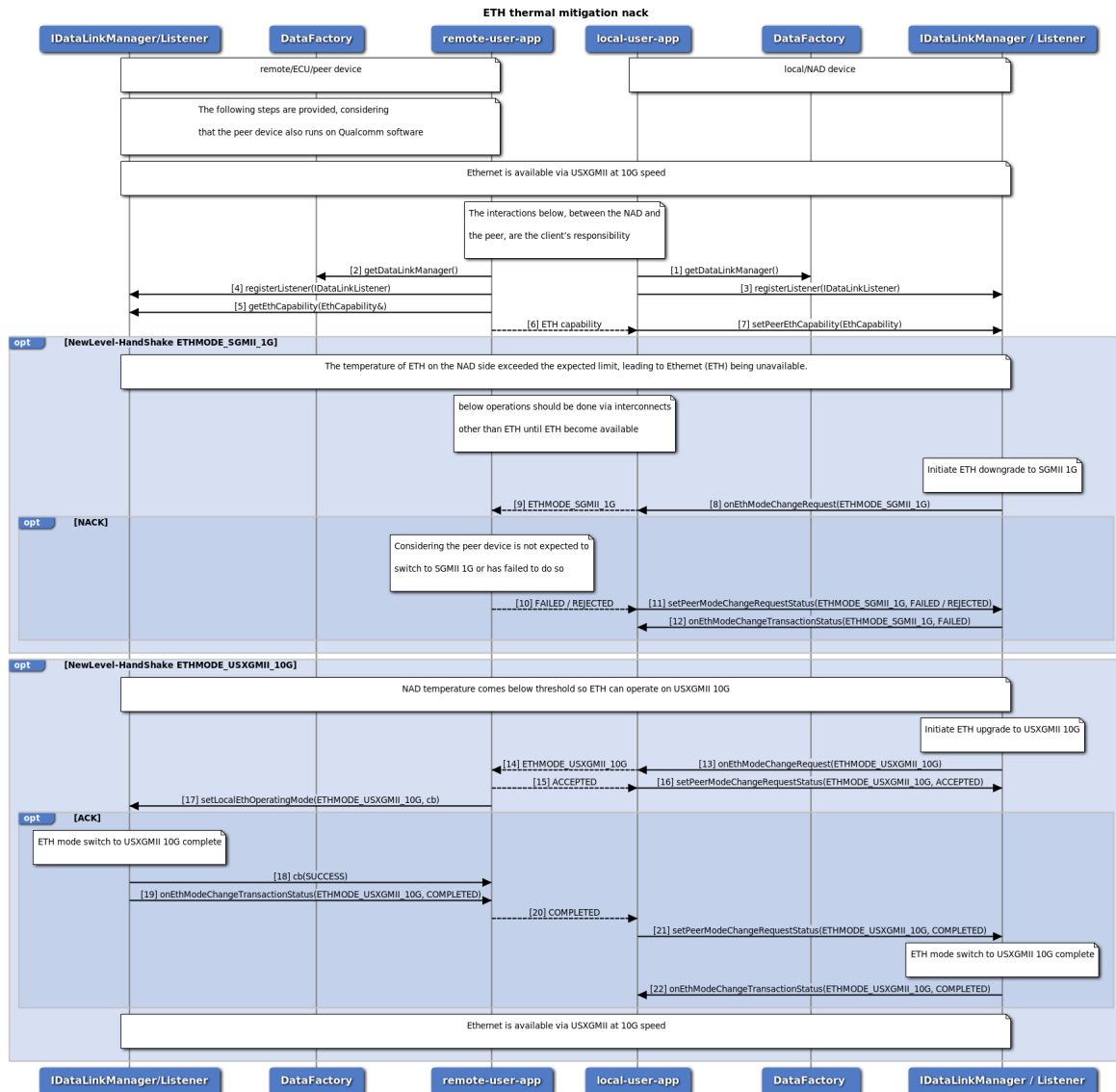
Figure 3-77 Call flow to update ETH mode as result of thermal mitigation nack
