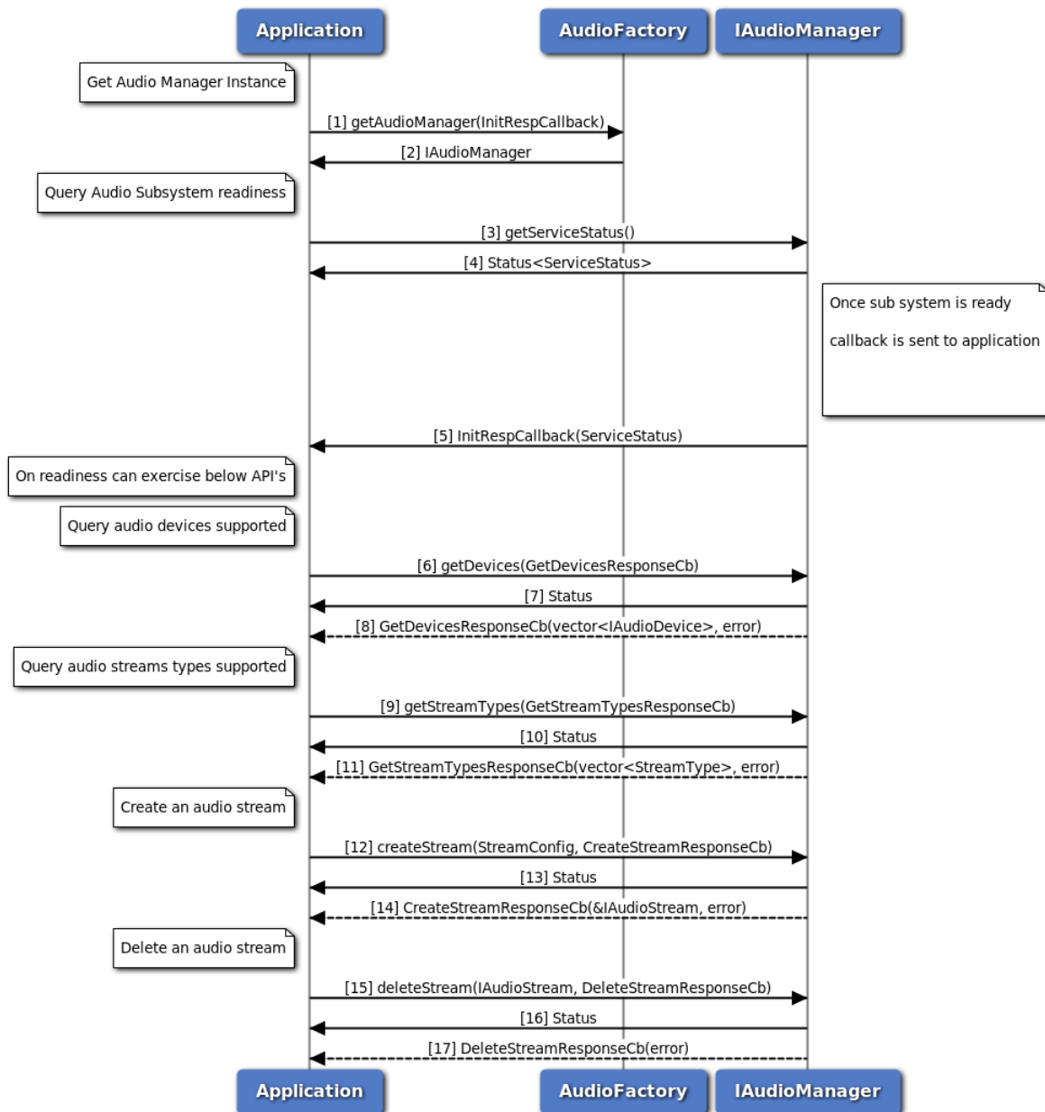
Figure 3-103 Audio Manager API call flow
