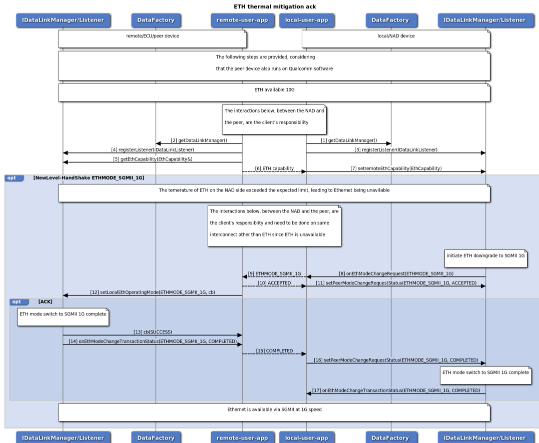
Figure 3-76 Call flow to update ETH mode as result of thermal mitigation
