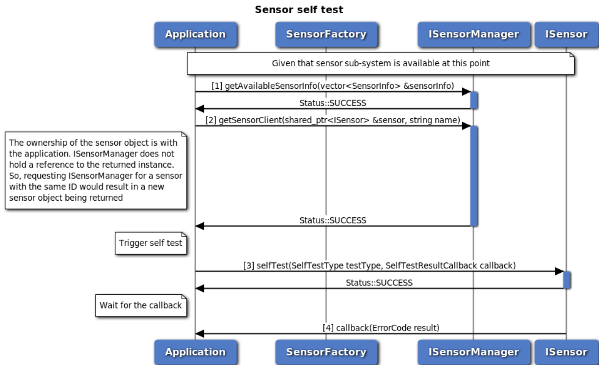
Figure 3-137 Sensor self test call flow
