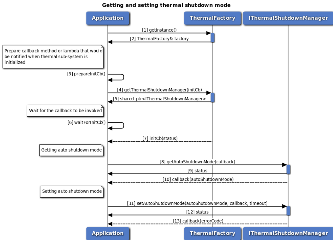
Figure 3-121 Call flow to set/get the Thermal auto-shutdown mode
