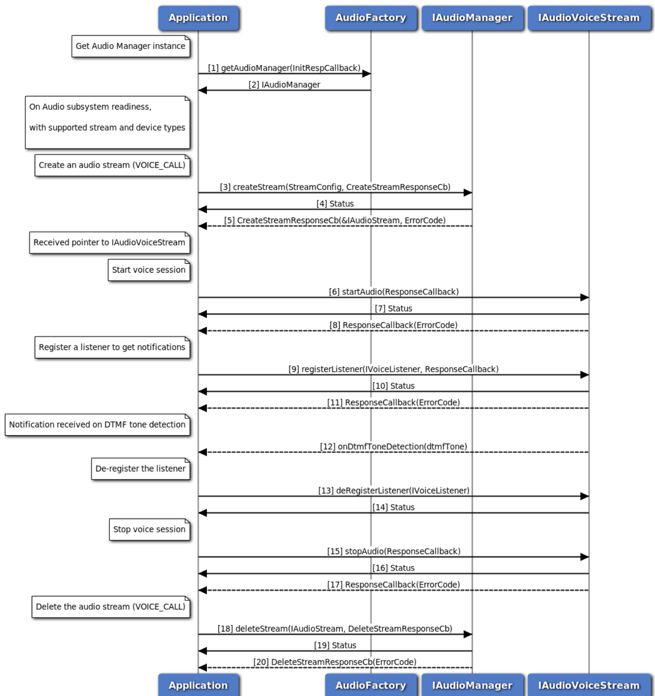
Figure 3-108 Call flow to detect DTMF tone
