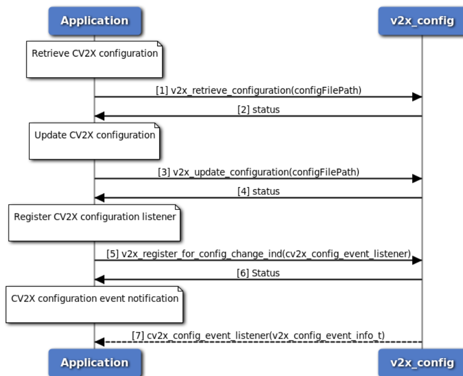
Figure 3-80 Retrieve/Update C-V2X Configuration Call Flow - C Version
