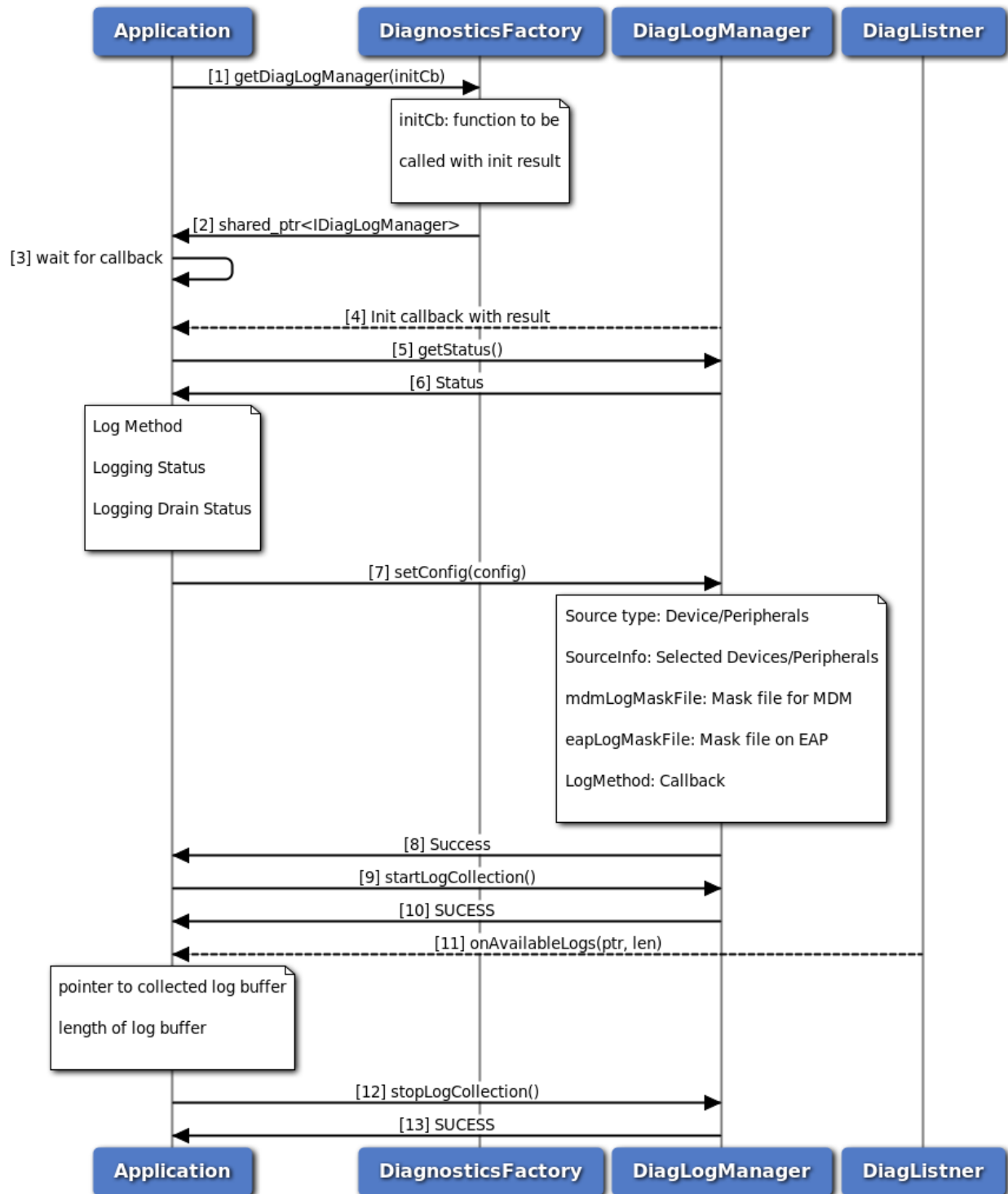
Figure 3-155 Log Collection Using Callback Method Call Flow
