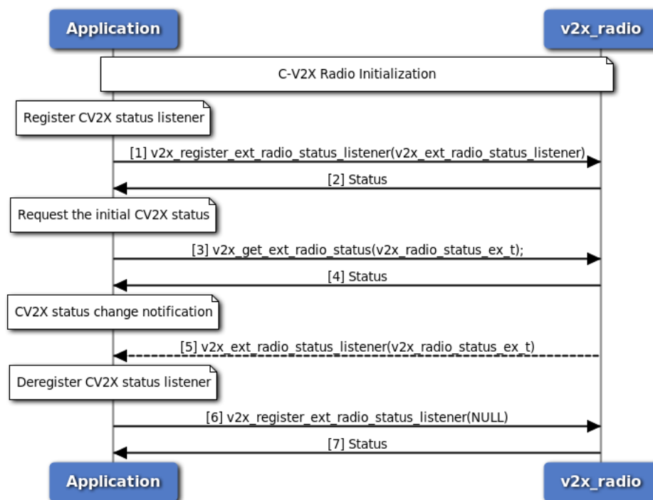
Figure 3-88 Get C-V2X Status Call Flow - C Version
