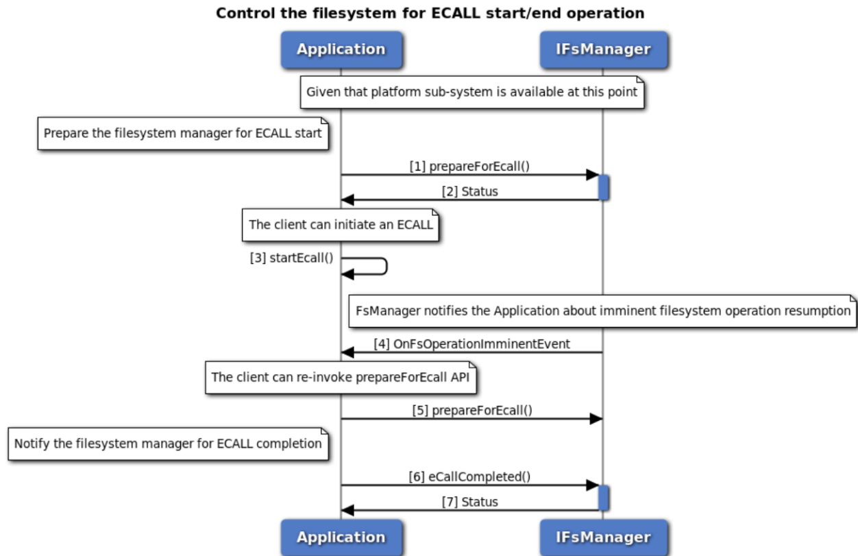
Figure 3-135 Control the filesystem for ECALL operation call flow
