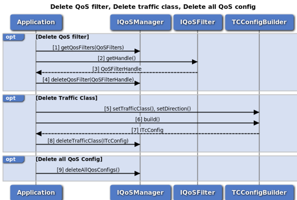
Figure 3-75 Delete QoS filter, Delete traffic class, Delete all QoS config
