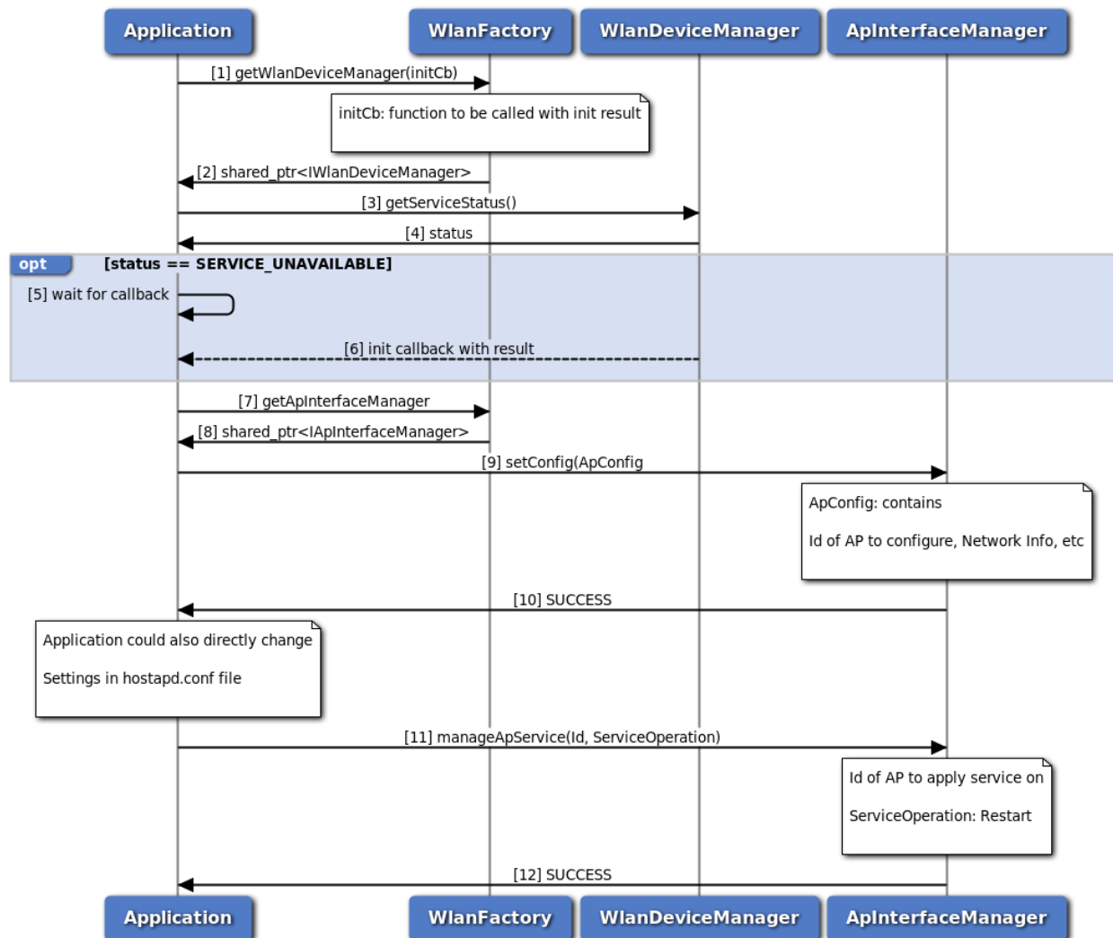
Figure 3-151 Modify WLAN Access Point Configuration Call Flow
