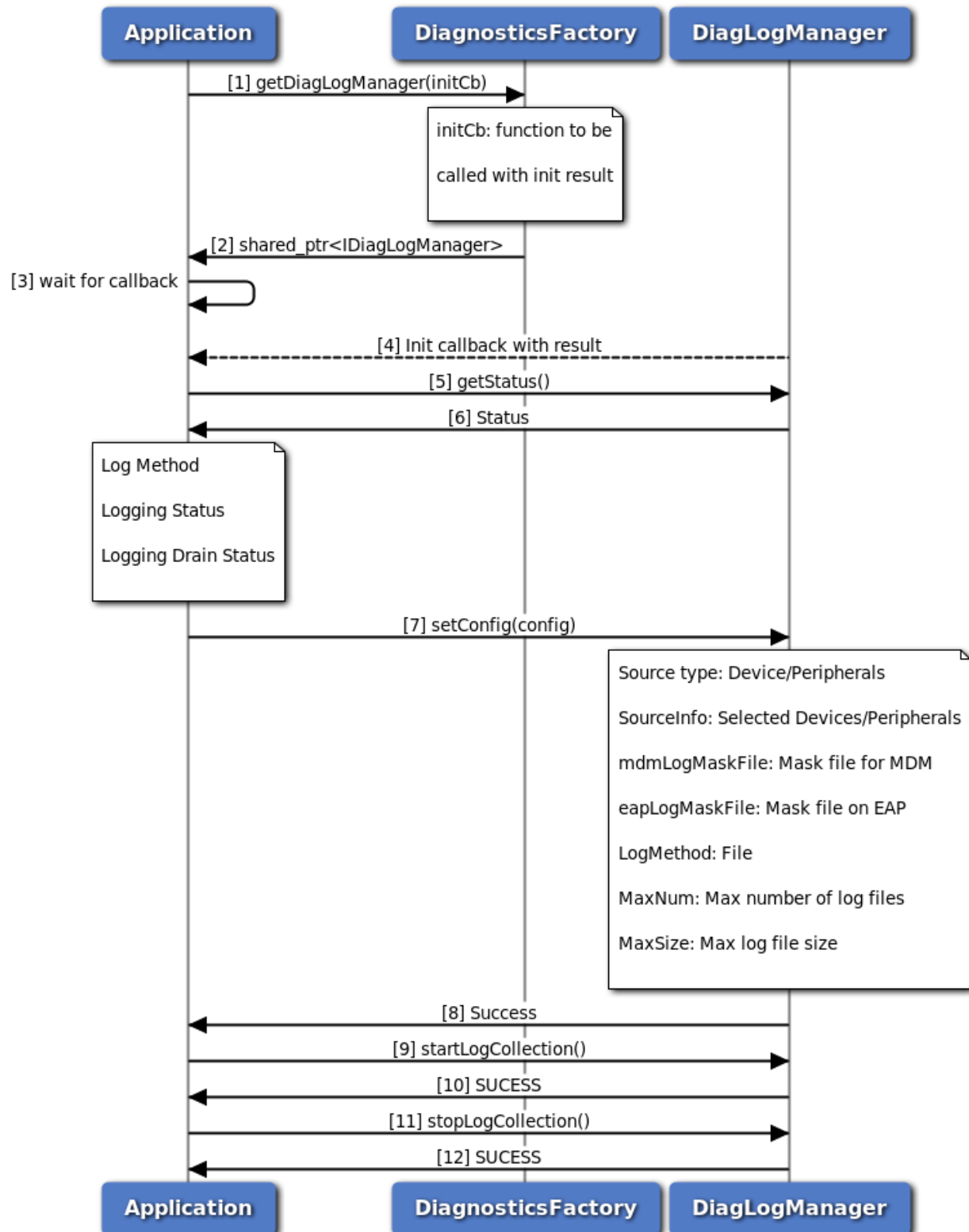
Figure 3-154 Log Collection Using File Method Call Flow
