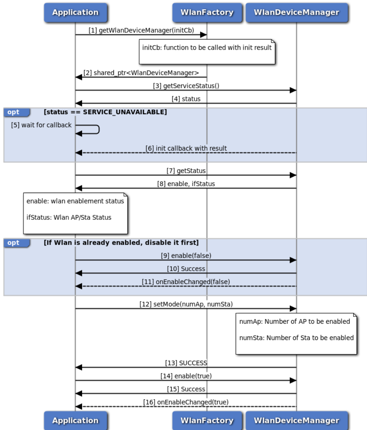
Figure 3-149 Modify WLAN Configuration Call Flow
