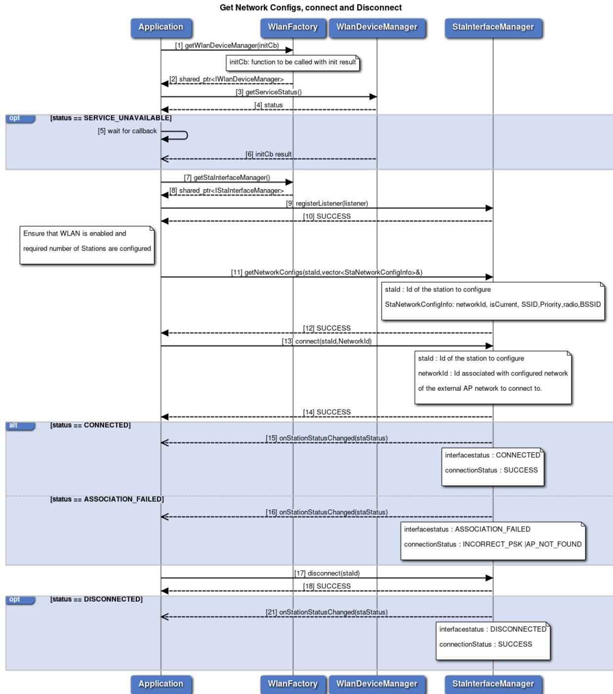
Figure 3-153 Get network configs, connect and disconnect
