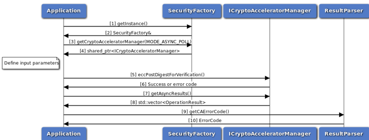
Figure 3-142 Call flow for signature verification asynchronous poll mode
