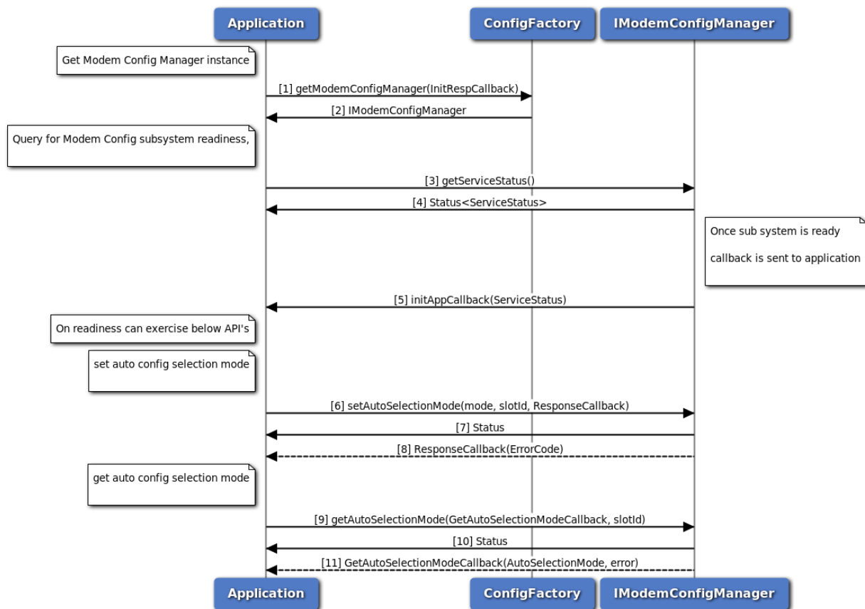
Figure 3-127 Modem Config get and set Auto Selection Mode Call Flow
