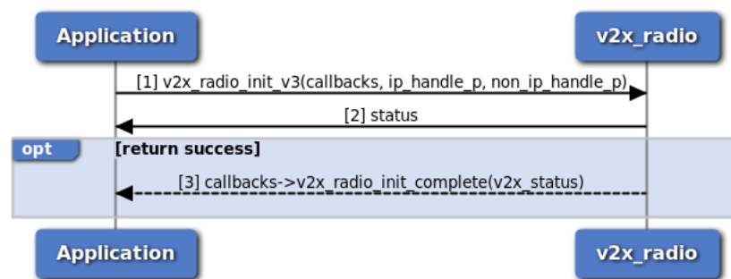
Figure 3-86 C-V2X Radio Initialization Call Flow - C Version
