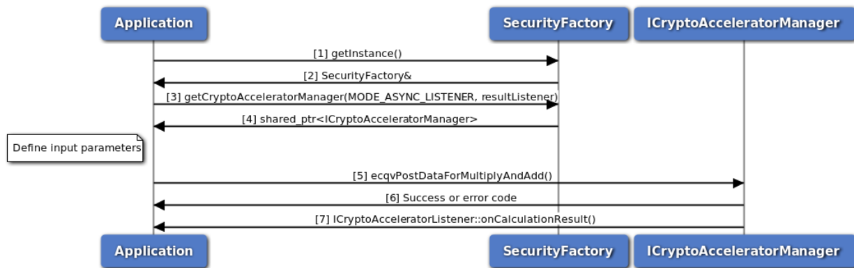
Figure 3-146 Call flow for ECQV calculation asynchronous listener mode
