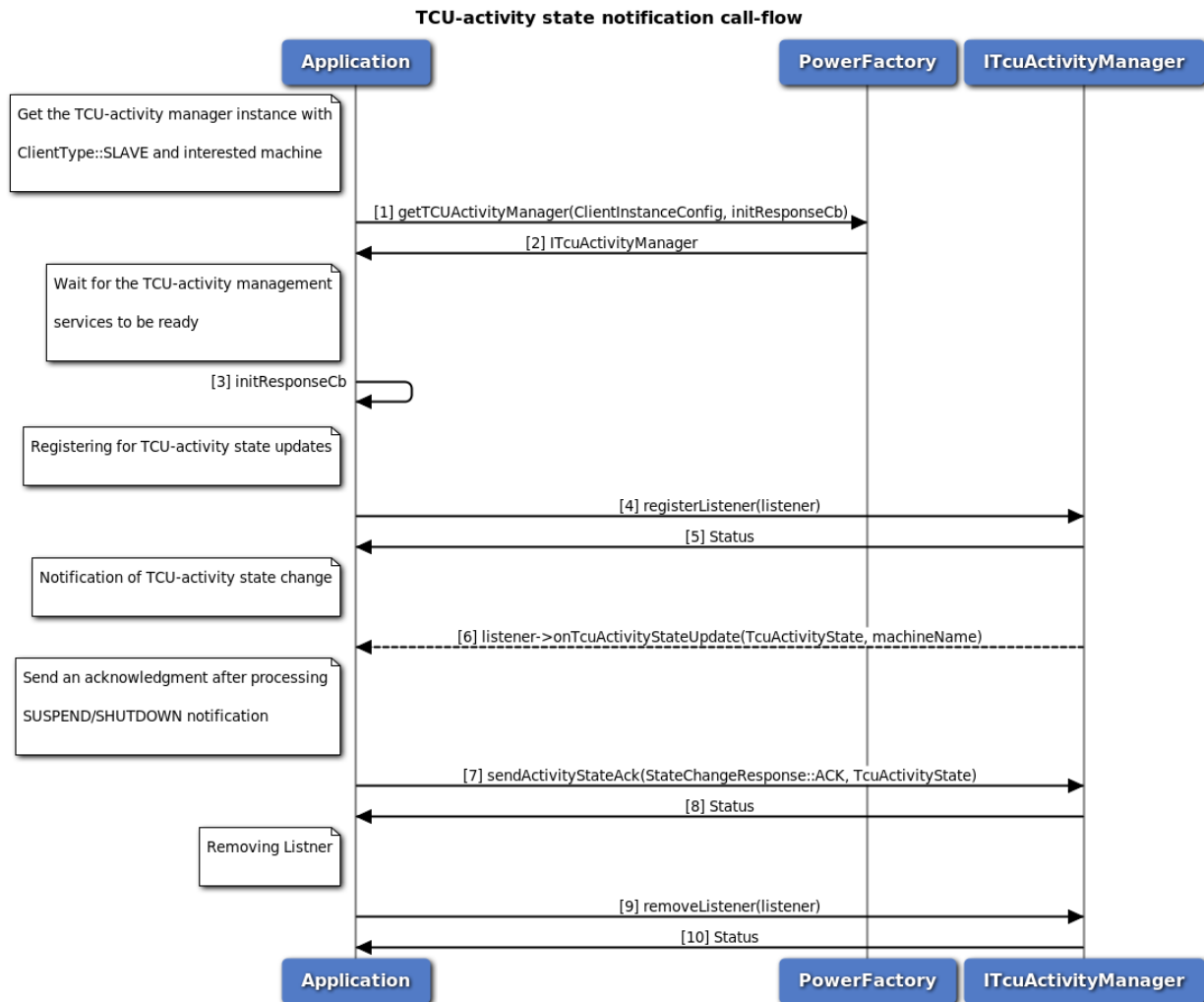
Figure 3-123 Call flow to register/remove listener for TCU-activity manager
