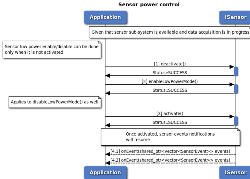
Figure 3-132 Sensor power control cleanup call flow
