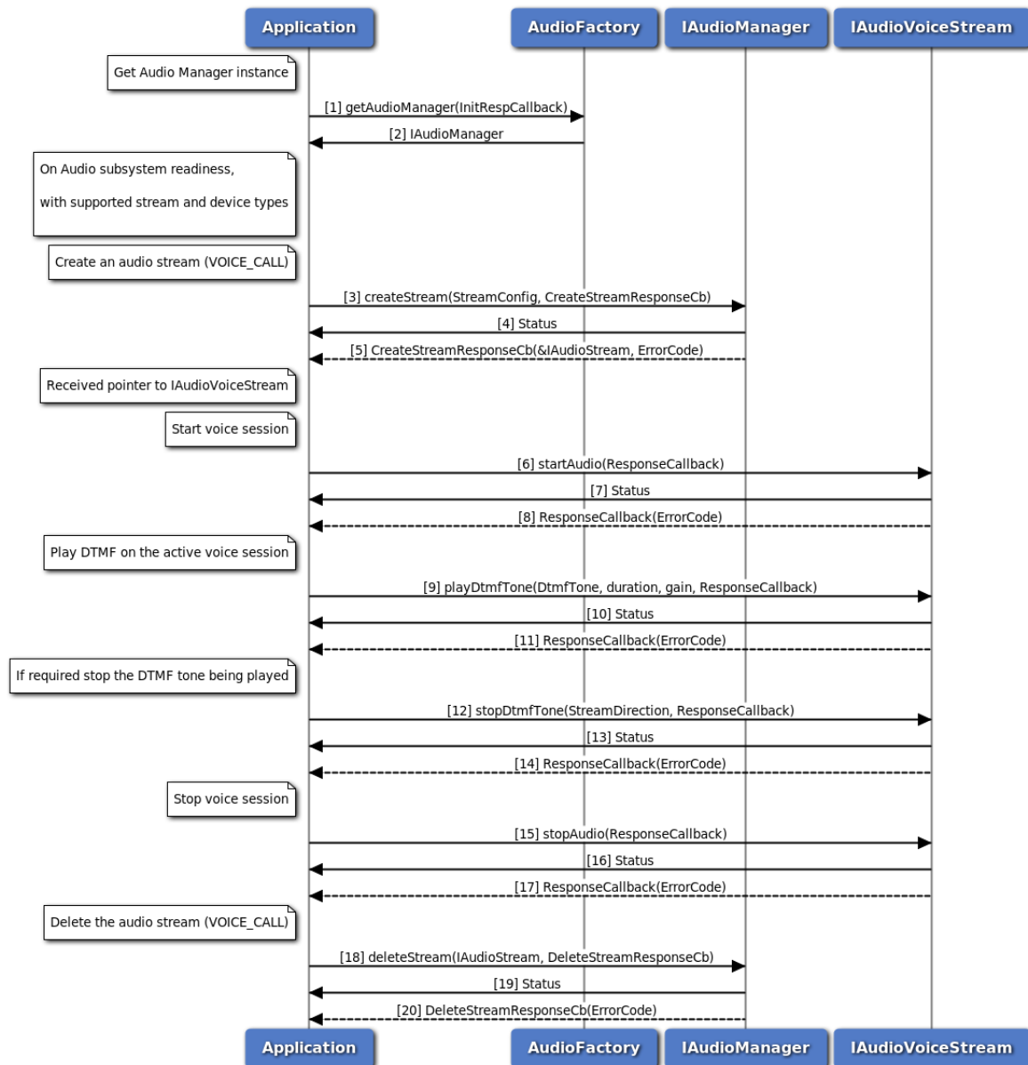
Figure 3-107 Call flow to play DTMF tone
