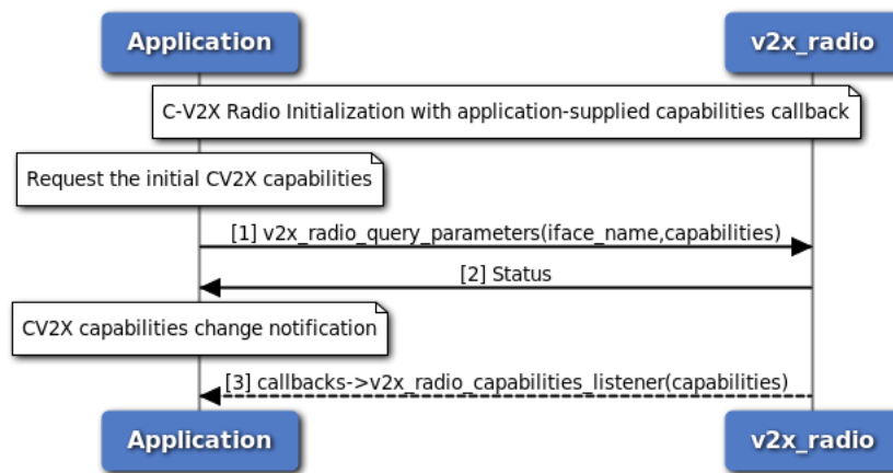
Figure 3-90 Get C-V2X Capabilities Call Flow - C Version
