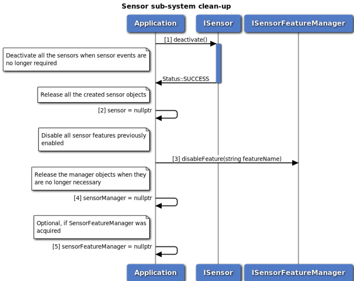
Figure 3-131 Sensor sub-system cleanup call flow
