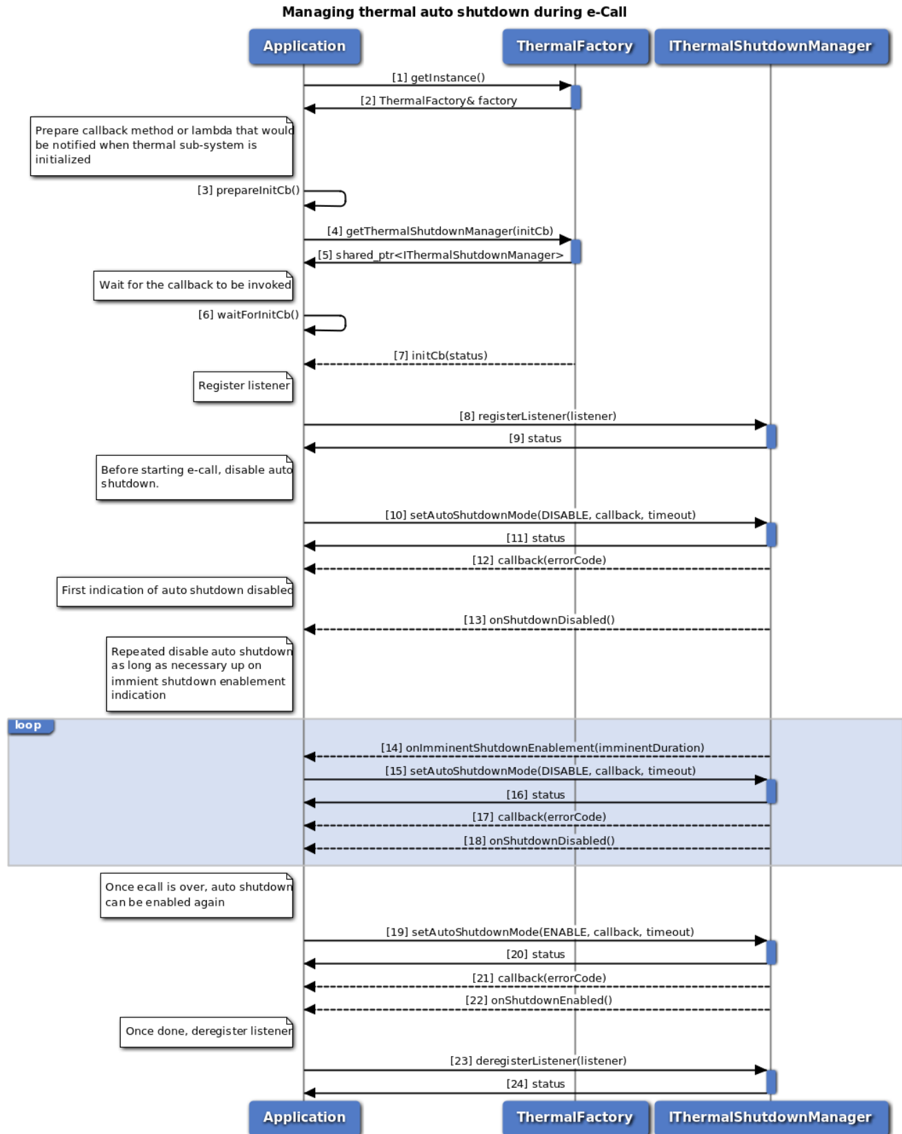
Figure 3-122 Call flow to manage thermal auto-shutdown from an eCall application
