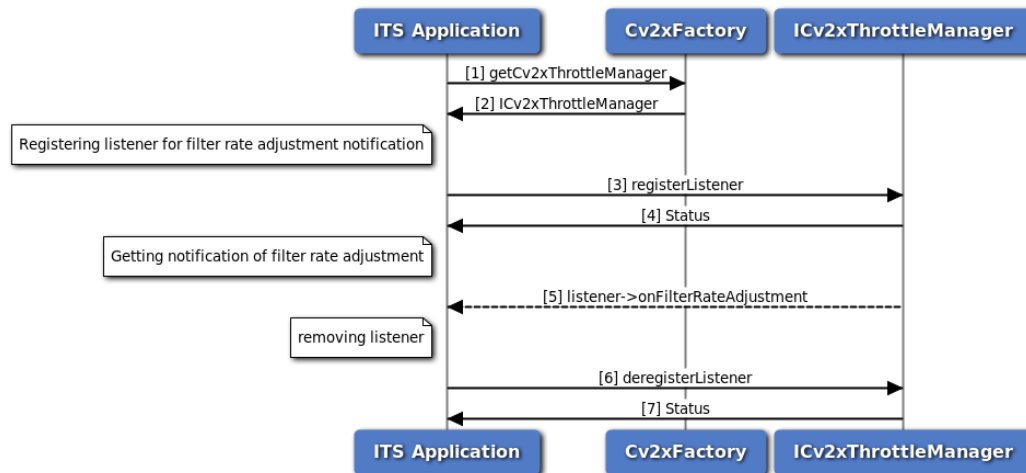
Figure 3-97 C-V2X Throttle Manager Filter Rate Adjustment Notification call flow
