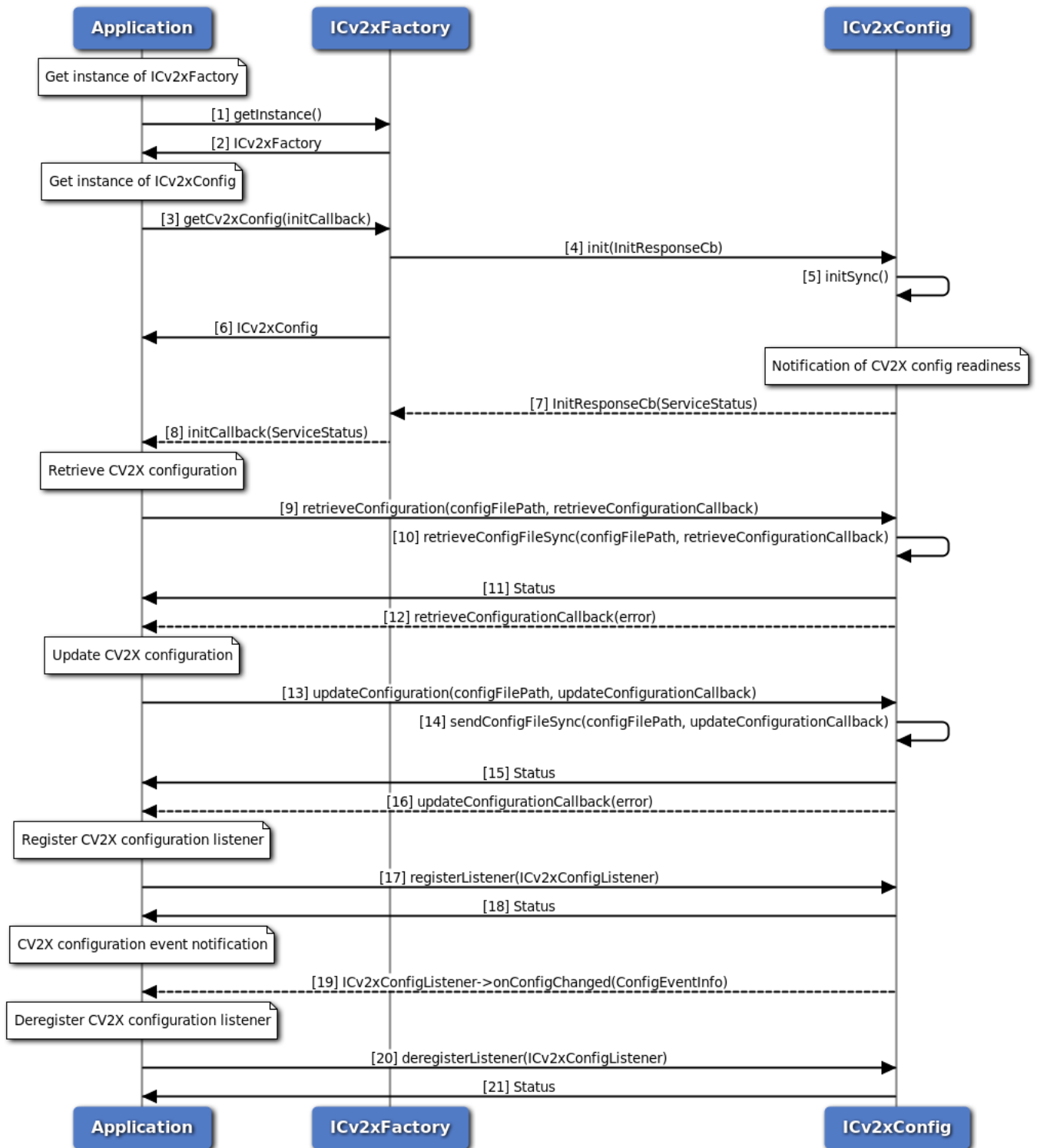
Figure 3-79 Retrieve/Update C-V2X Configuration Call Flow - C++ version
