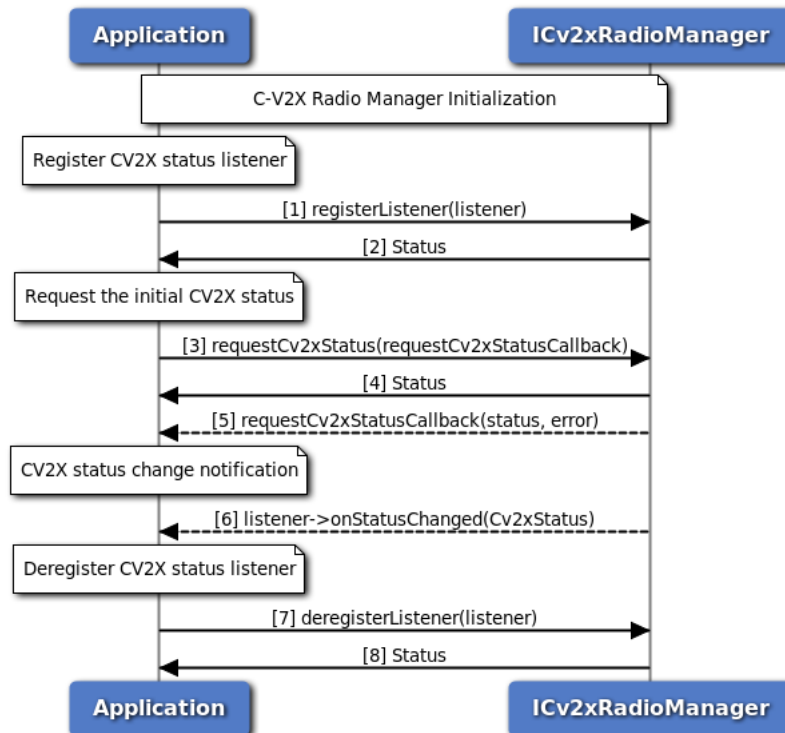
Figure 3-87 Get C-V2X Status Call Flow - C++ Version
