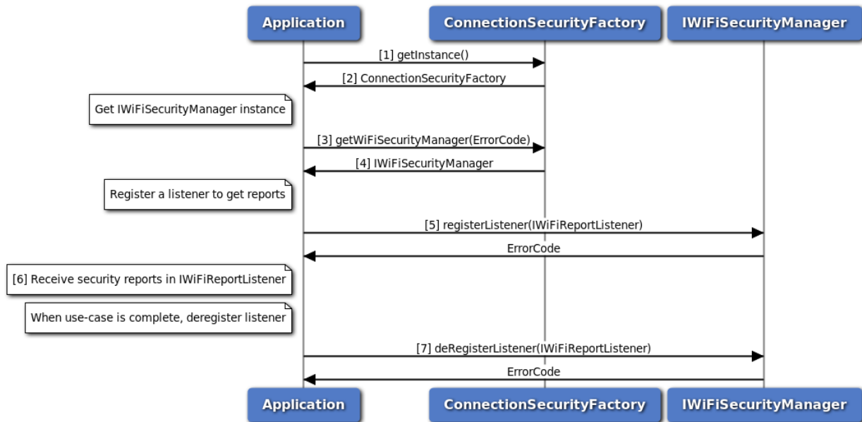
Figure 3-148 Call flow to register listener and receive reports
