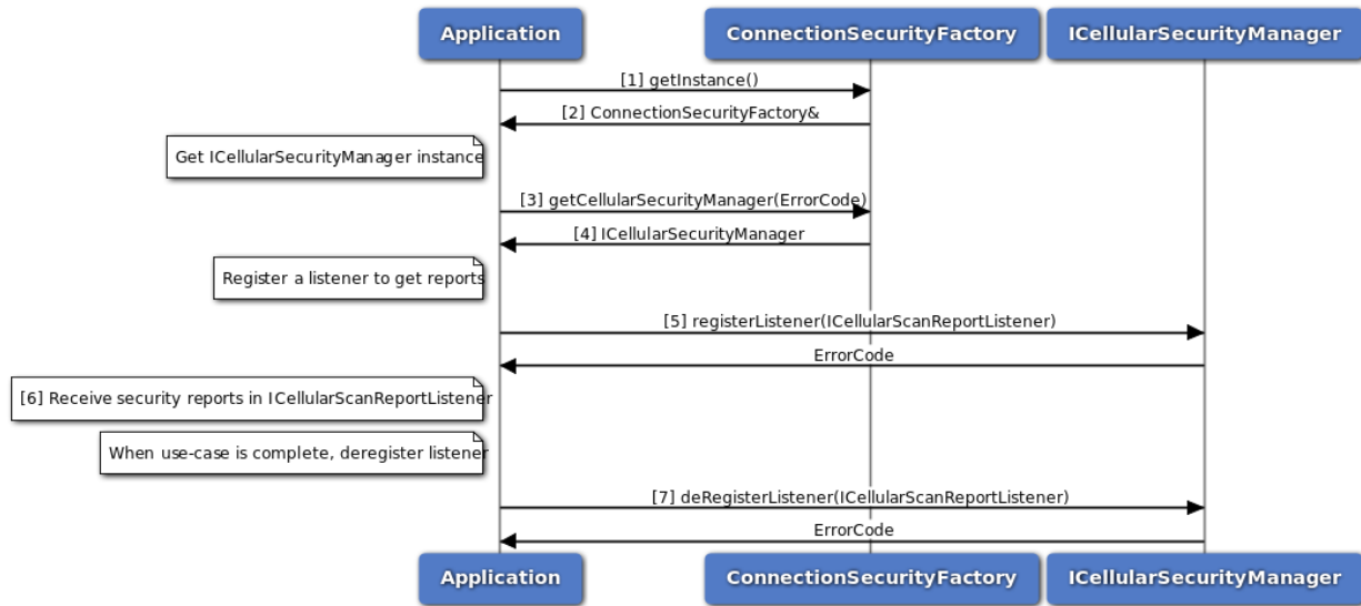
Figure 3-147 Call flow to register listener and receive reports
