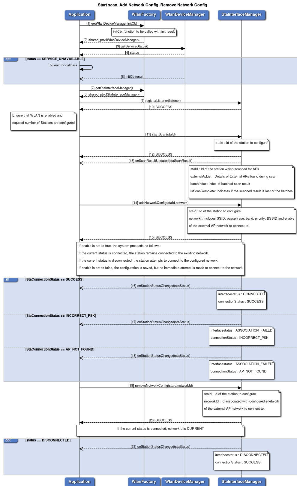
Figure 3-152 start scan, add network config, or remove network config
