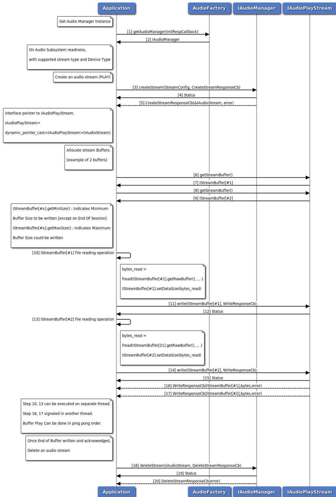
Figure 3-109 Audio Playback call flow
