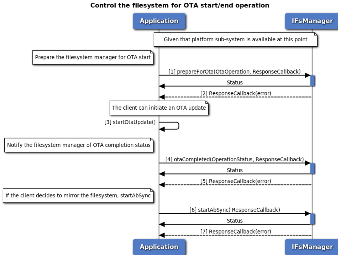
Figure 3-136 Control the filesystem for OTA operation call flow
