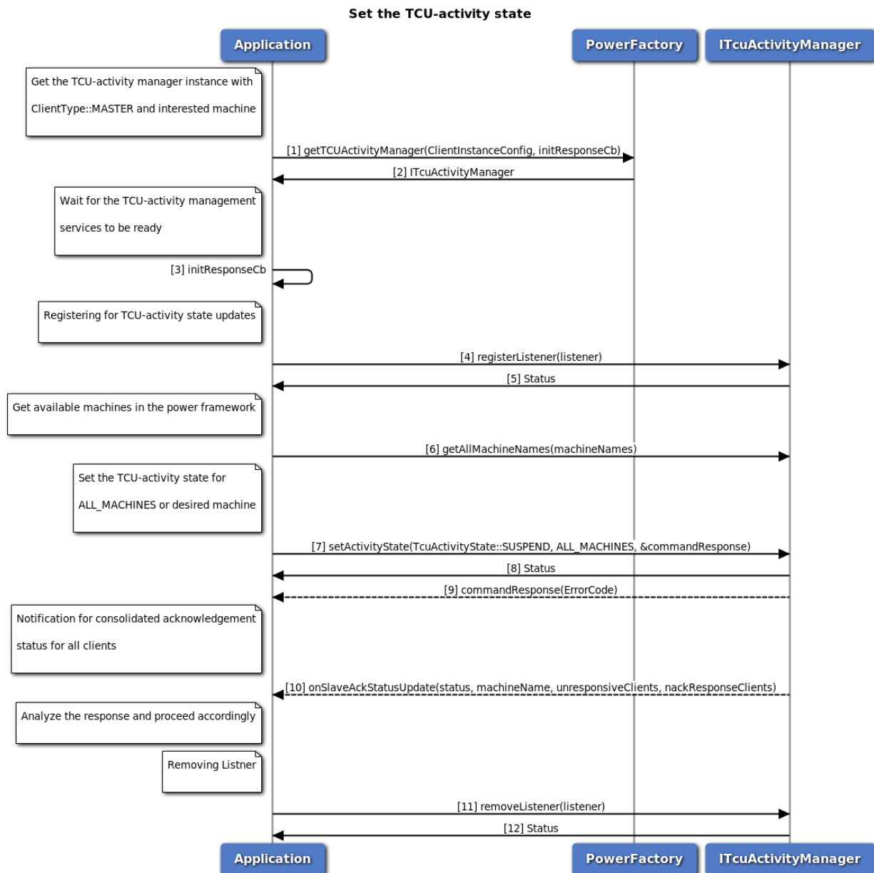
Figure 3-124 Call flow to set the TCU-activity state
