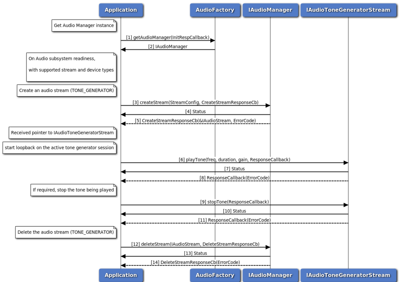
Figure 3-111 Call flow to play/stop tone on a sink device
