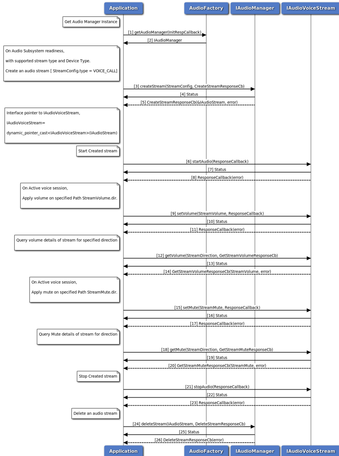
Figure 3-106 Audio Voice Call Volume/Mute control call flow
