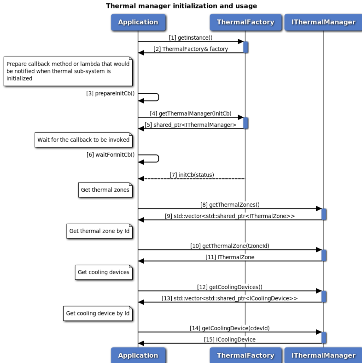
Figure 3-118 Thermal manager API call flow
