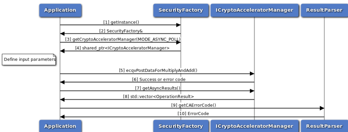
Figure 3-145 Call flow for ECQV calculation asynchronous poll mode
