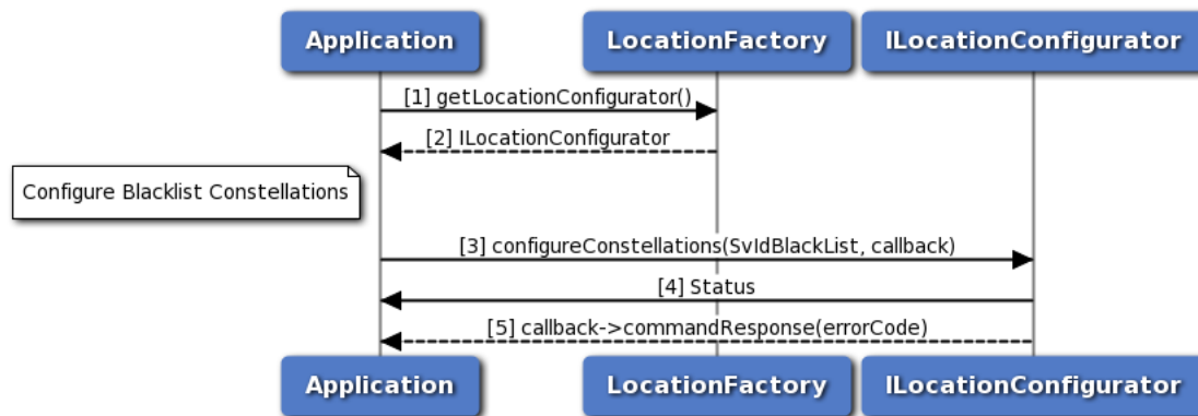
Figure 3-30 Call flow to configure blacklisted constellations
