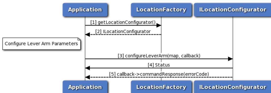
Figure 3-29 Call flow to configure lever arm parameters
