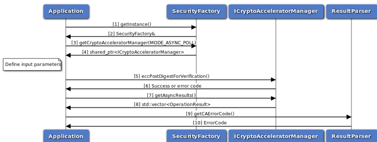
Figure 3-135 Call flow for signature verification asynchronous poll mode
