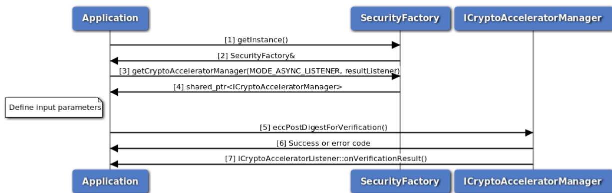
Figure 3-136 Call flow for signature verification asynchronous listener mode
