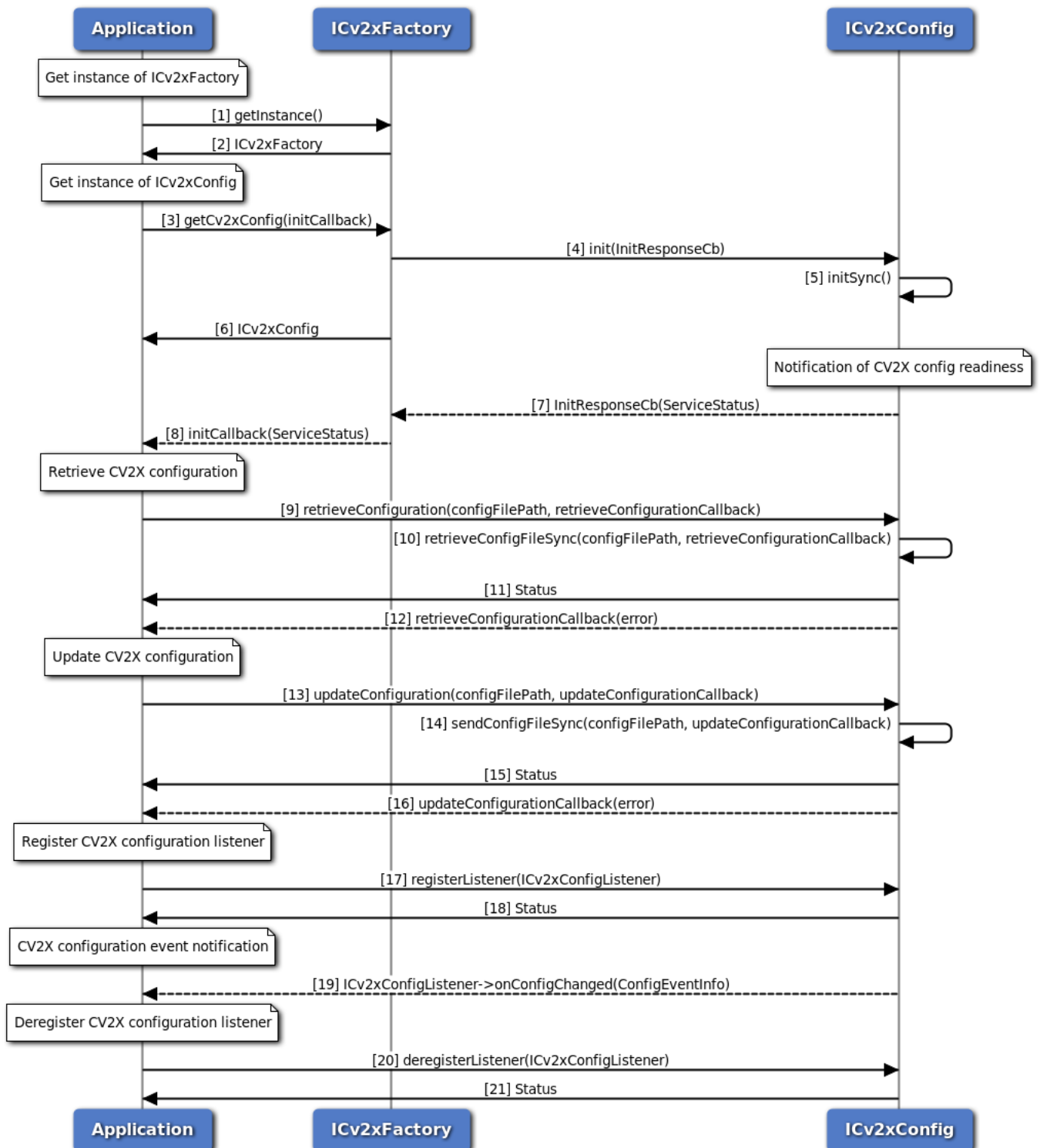
Figure 3-72 Retrieve/Update C-V2X Configuration Call Flow - C++ version
