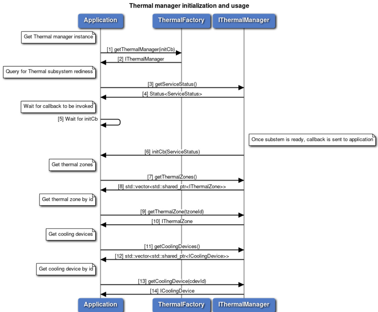
Figure 3-111 Thermal manager call flow
