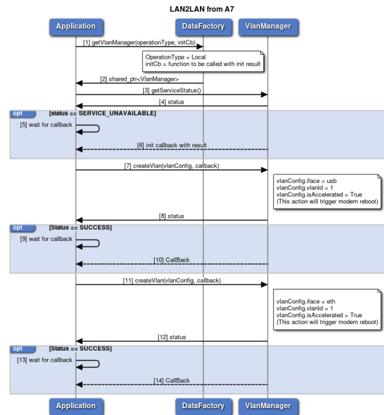
Figure 3-61 LAN-LAN VLAN Configuration Usecase from A7 call flow
