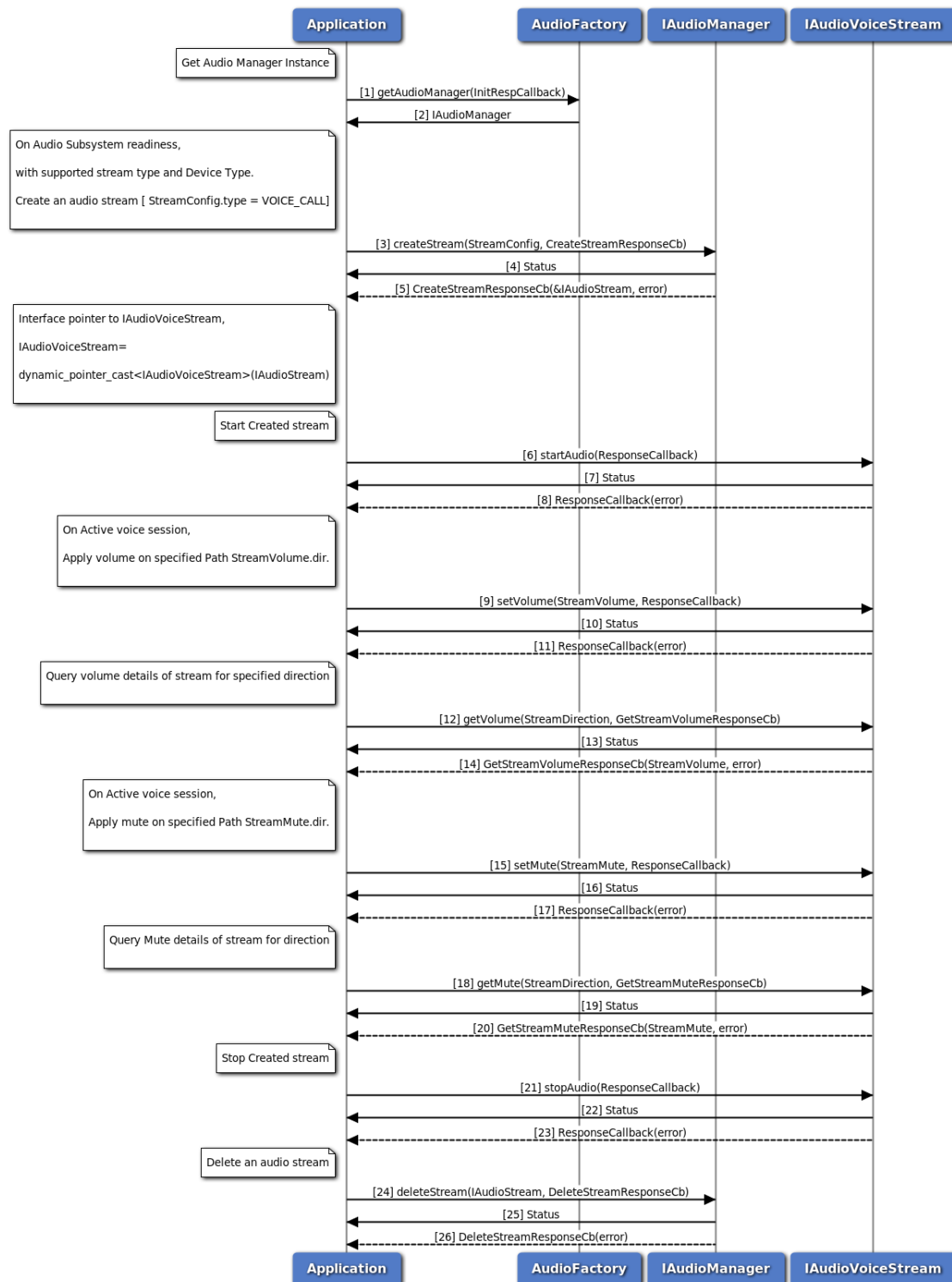
Figure 3-99 Audio Voice Call Volume/Mute control call flow
