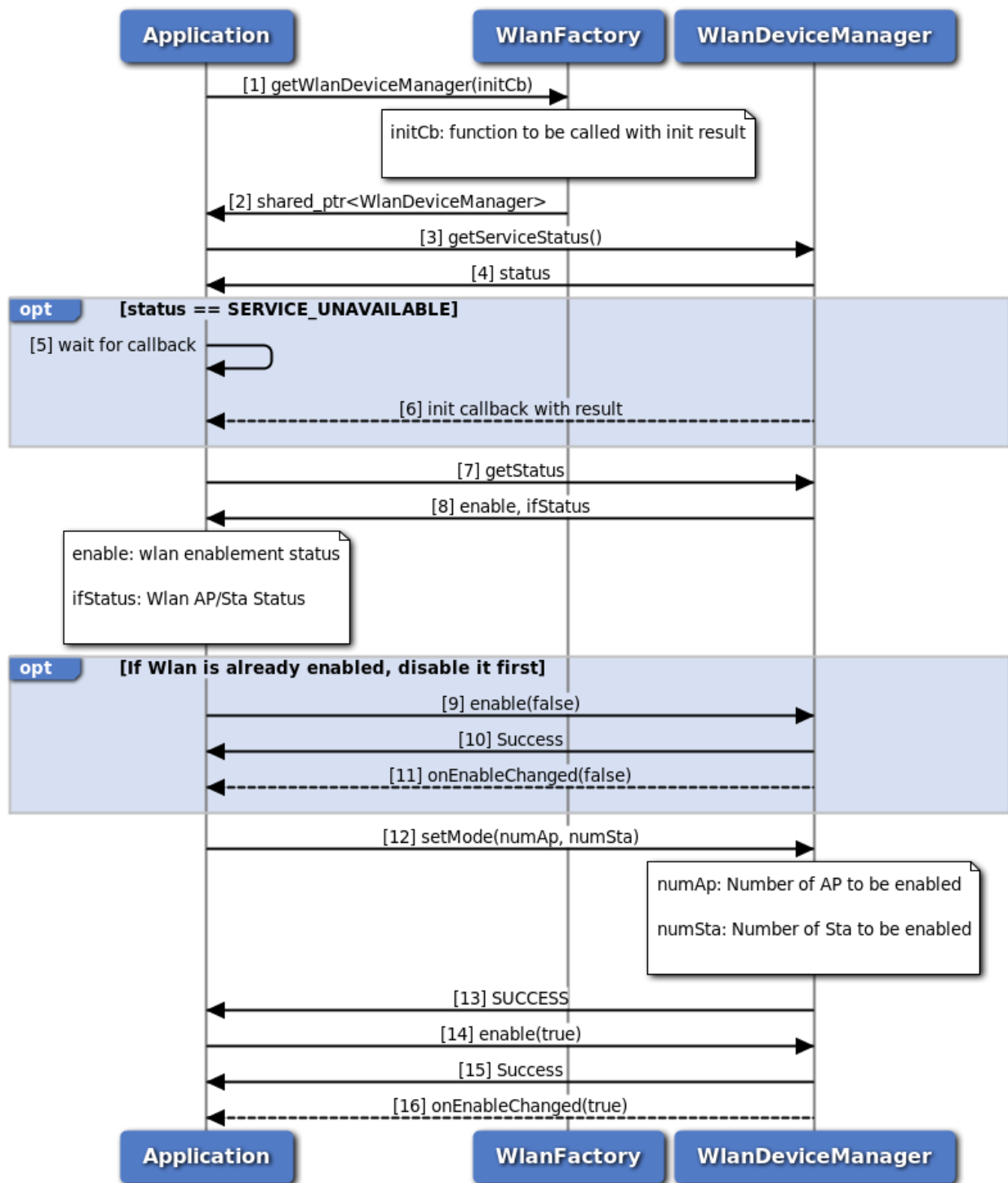
Figure 3-140 Modify WLAN Configuration Call Flow
