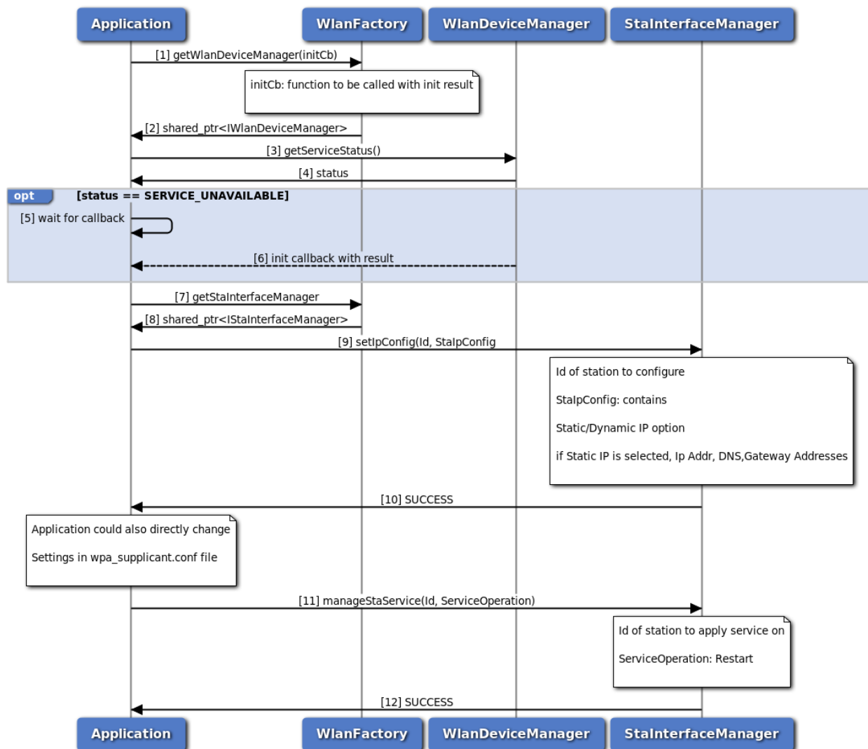
Figure 3-141 Modify WLAN Station Configuration Call Flow
