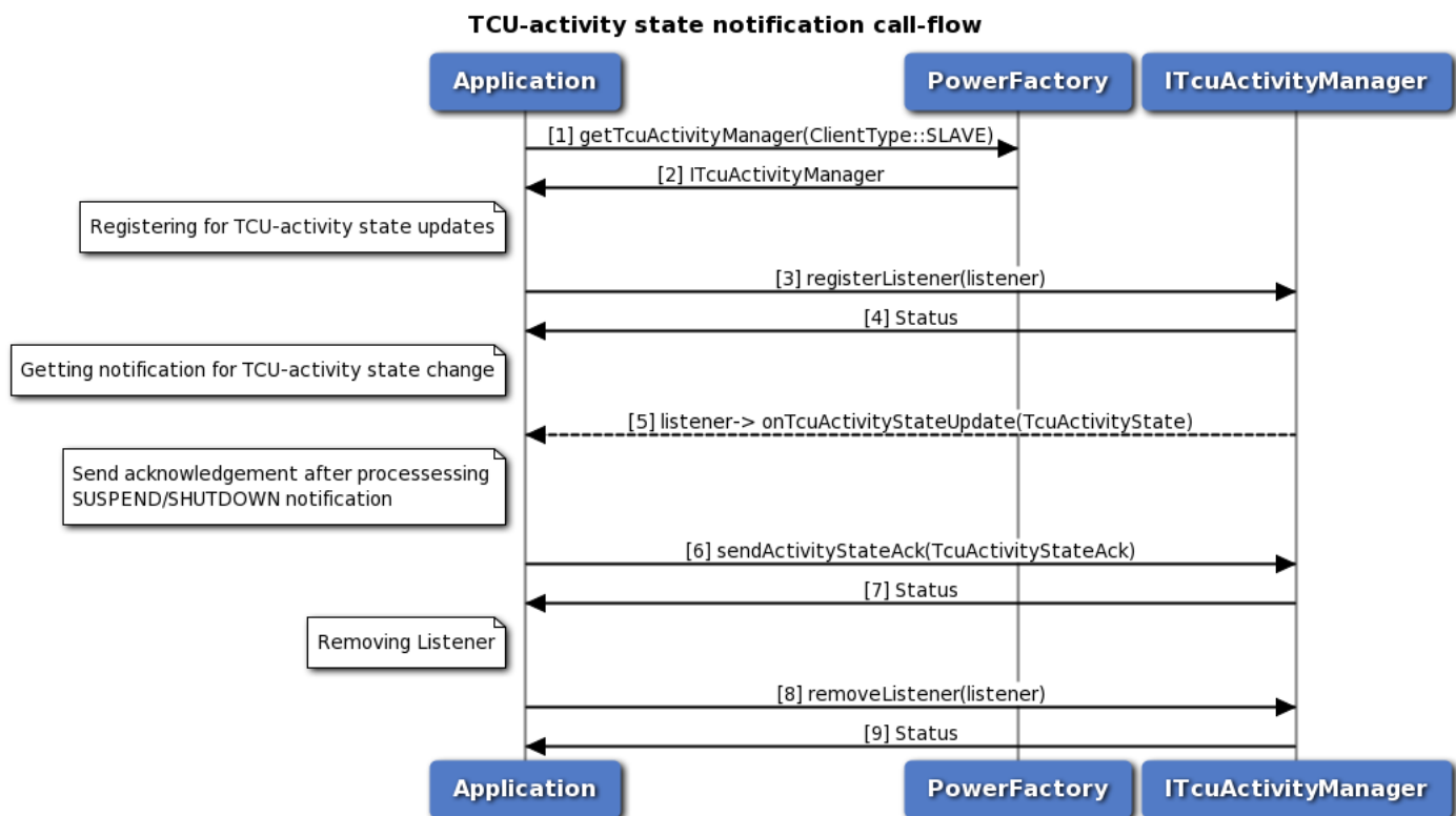
Figure 3-115 Call flow to register/remove listener for TCU-activity manager
