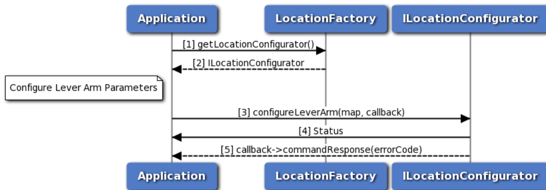
Figure 3-34 Call flow to configure lever arm parameters
