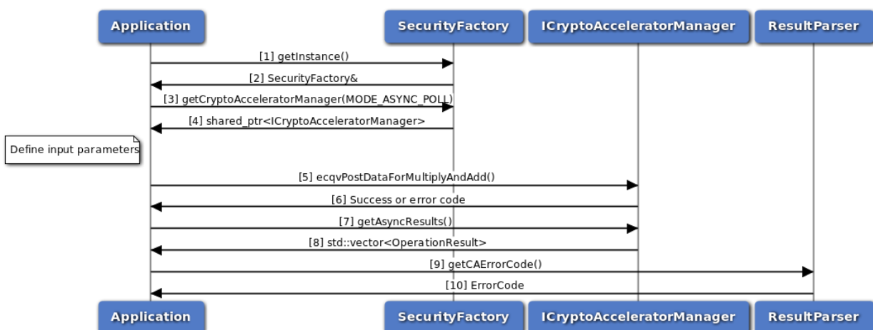
Figure 3-138 Call flow for ECQV calculation asynchronous poll mode
