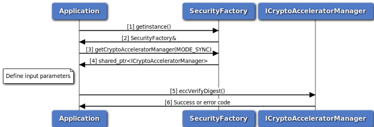
Figure 3-134 Call flow for signature verification synchronous mode
