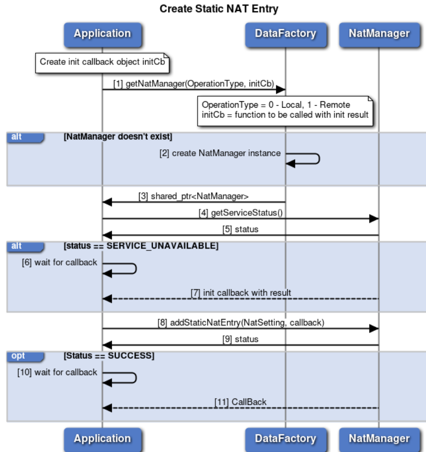
Figure 3-64 Create Static NAT entry for data NAT manager call flow
