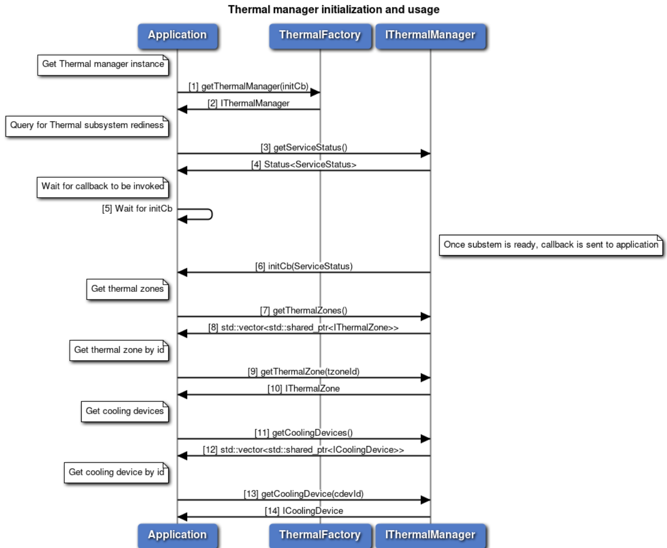
Figure 3-112 Thermal manager call flow
