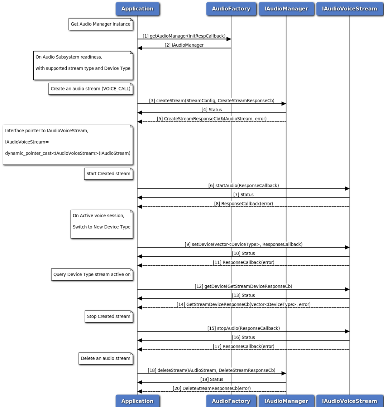
Figure 3-99 Audio Voice Call Device Switch call flow
