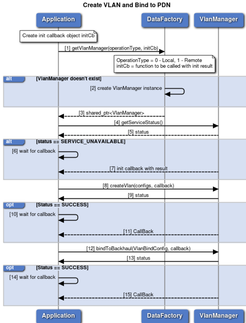
Figure 3-59 Create VLAN and bind it to PDN for data VLAN manager call flow
