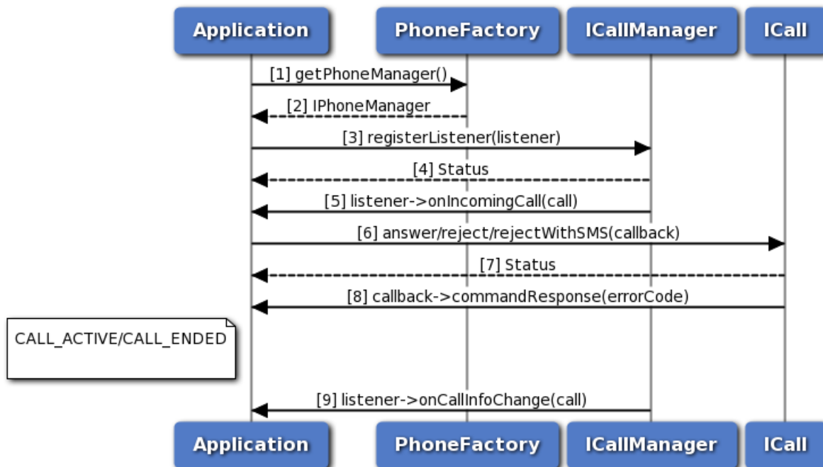
Figure 3-6 Answer, Reject call flow
