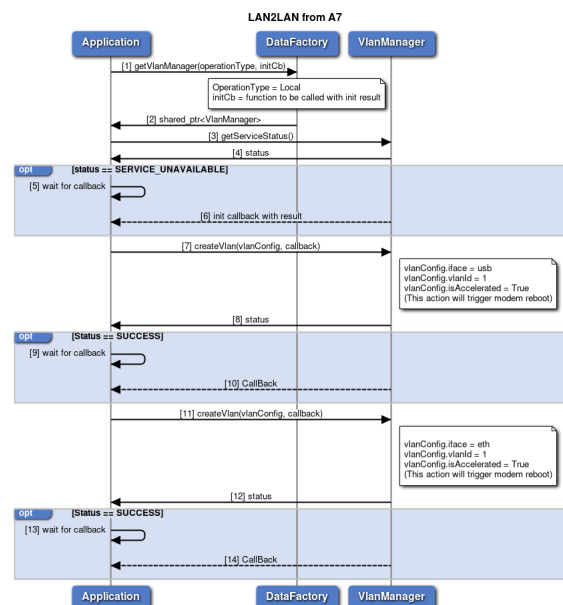
Figure 3-61 LAN-LAN VLAN Configuration Usecase from A7 call flow
