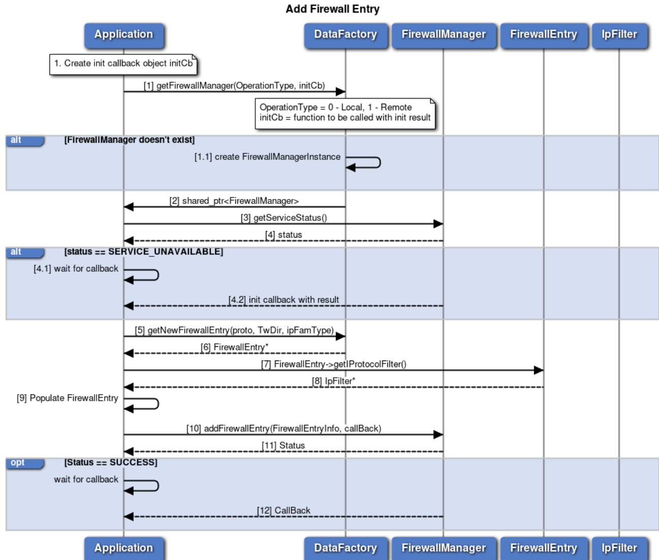
Figure 3-66 Add Firewall entry in data Firewall manager call flow
