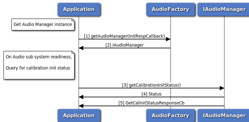
Figure 3-111 Audio calibration configuration status
