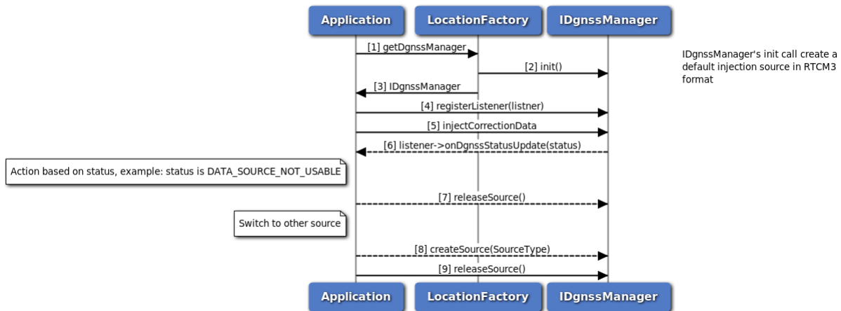
Figure 3-50 Call flow to inject RTCM correction data with dgnss manager
