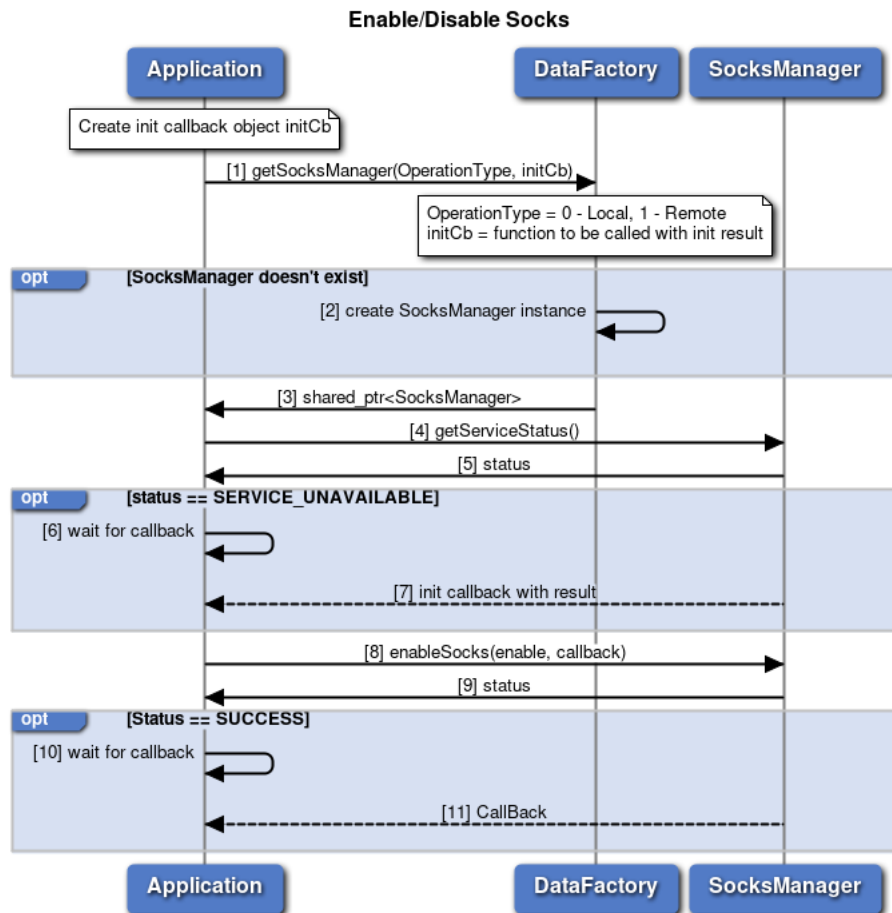
Figure 3-68 Socks enablement in data Socks manager call flow
