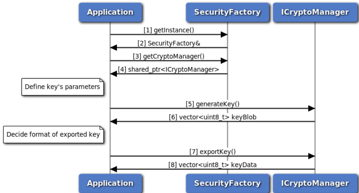
Figure 3-132 Call flow to generate and export key
