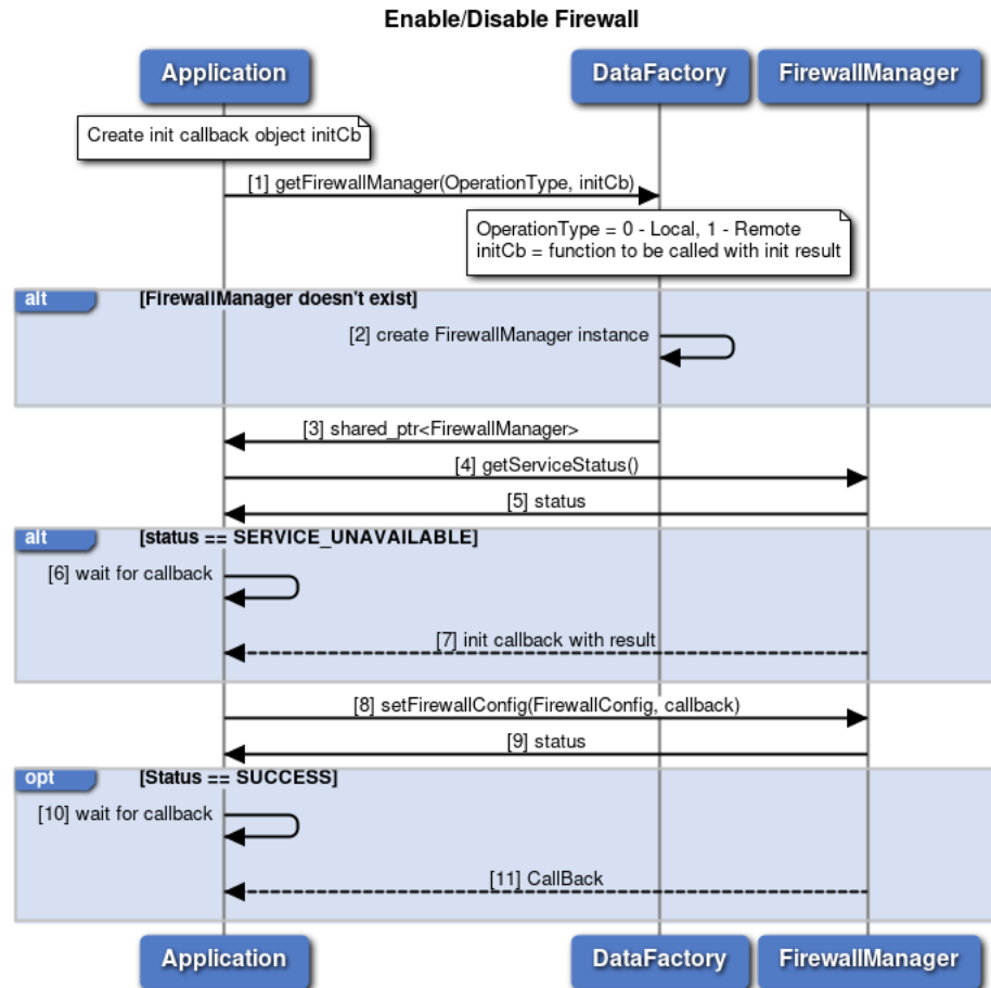
Figure 3-65 Firewall enablement in data Firewall manager call flow
