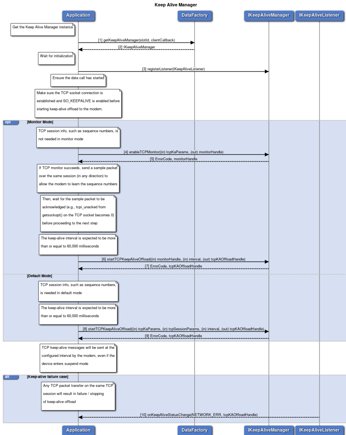
Figure 3-72 Call flow to start TCP keep alive offload to modem
