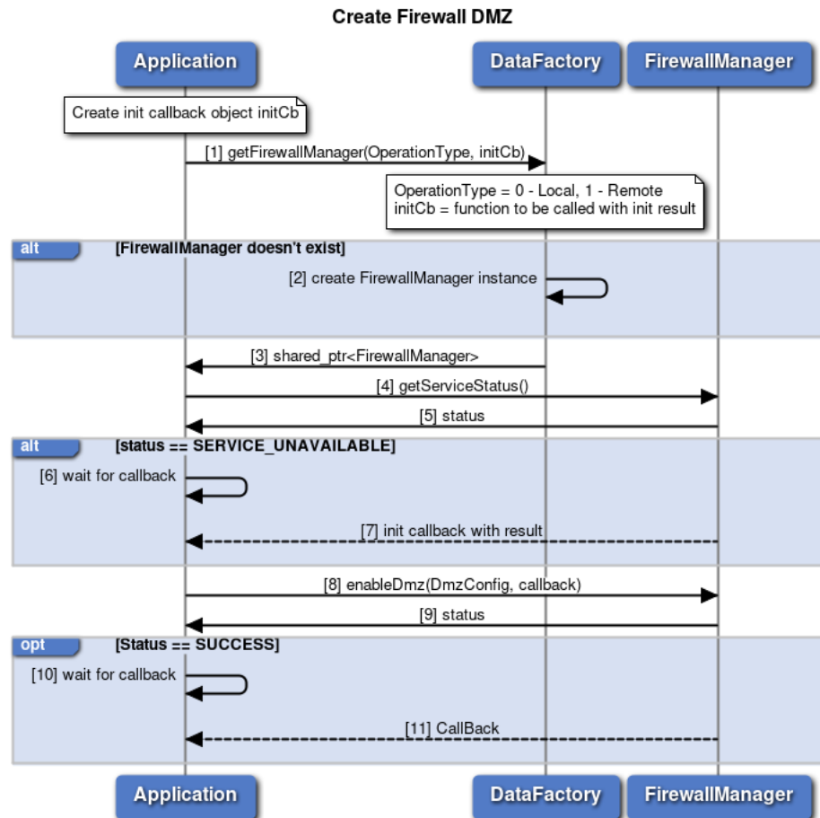
Figure 3-67 Set Firewall DMZ in data Firewall manager call flow
