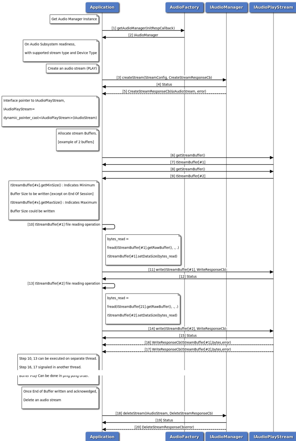
Figure 3-97 Audio Playback call flow
