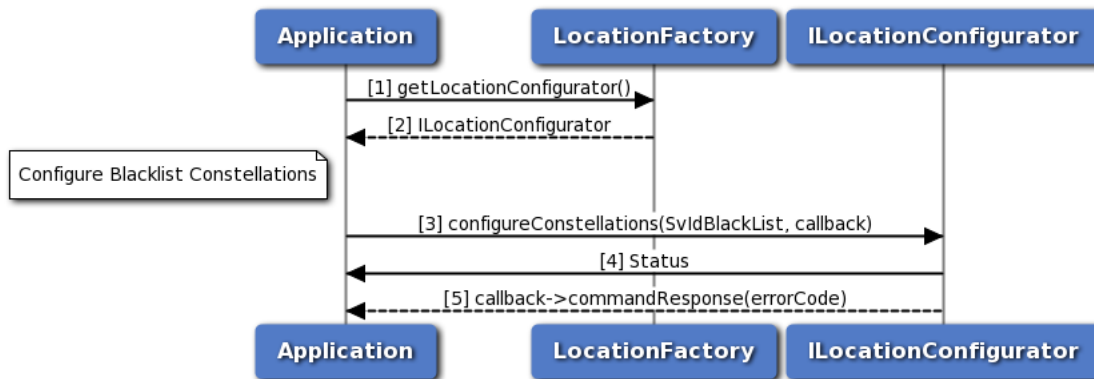
Figure 3-33 Call flow to configure blacklisted constellations
