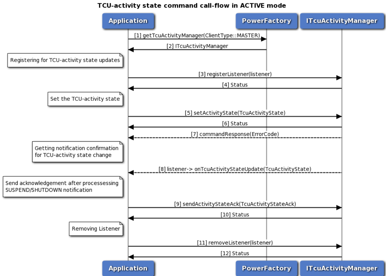
Figure 3-113 Call flow to set the TCU-activity state in ACTIVE mode
