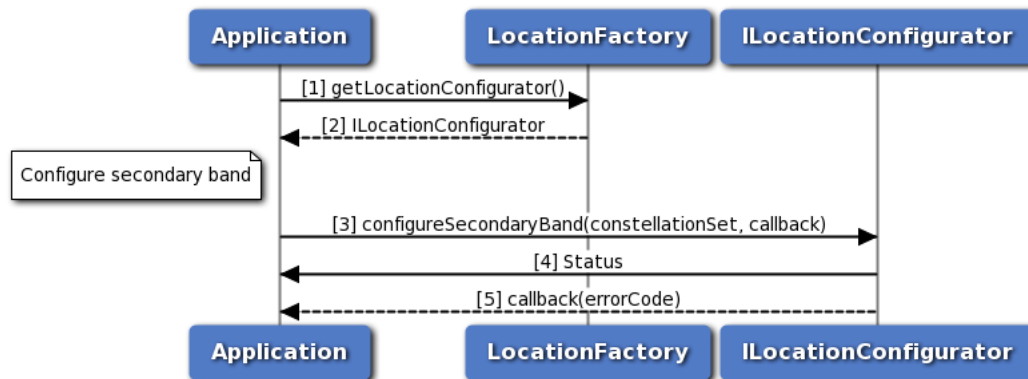
Figure 3-42 Call flow to configure secondary band
