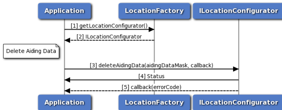
Figure 3-37 Call flow to delete specified data
