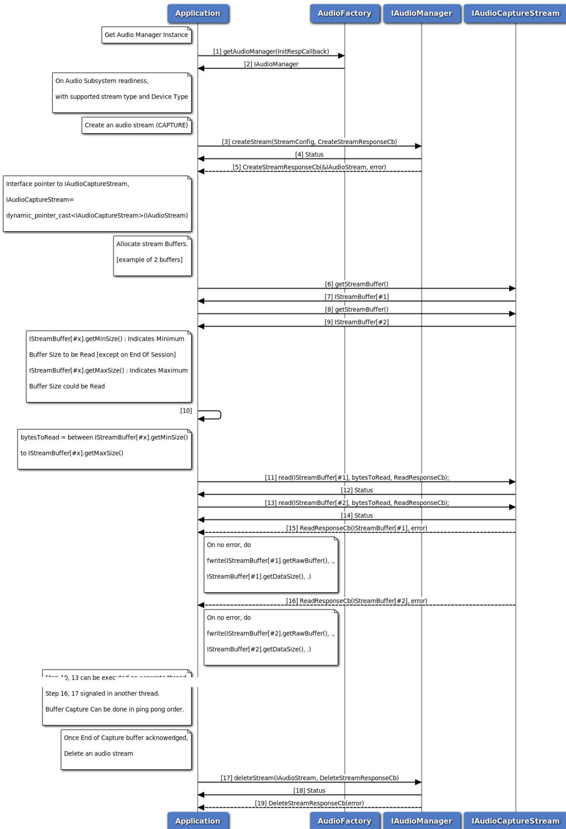
Figure 3-100 Audio Capture call flow
