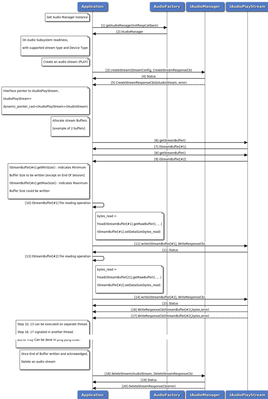
Figure 3-99 Audio Playback call flow
