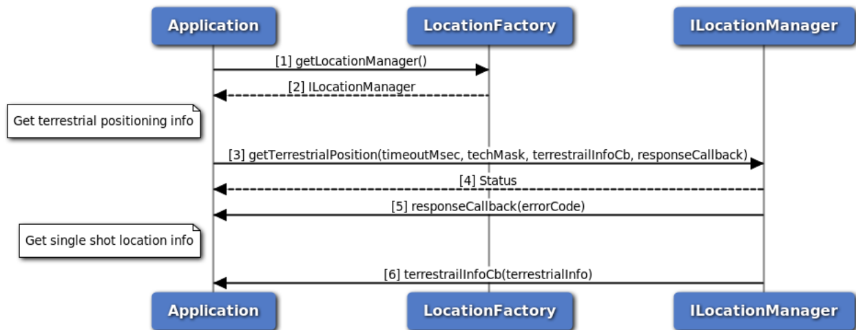
Figure 3-27 Call flow to get terrestrial positioning information
