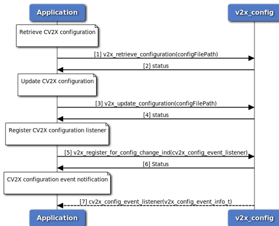
Figure 3-70 Retrieve/Update C-V2X Configuration Call Flow - C Version
