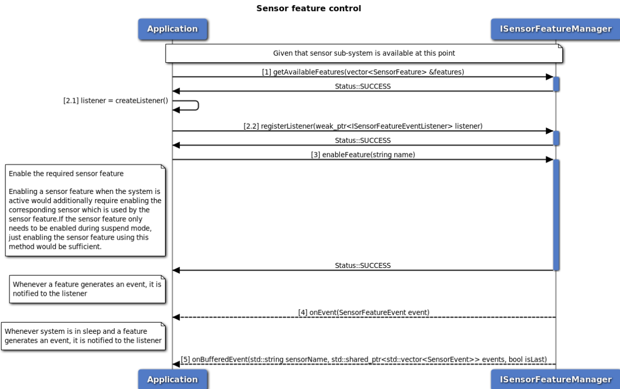
Figure 3-124 Sensor feature control cleanup call flow
