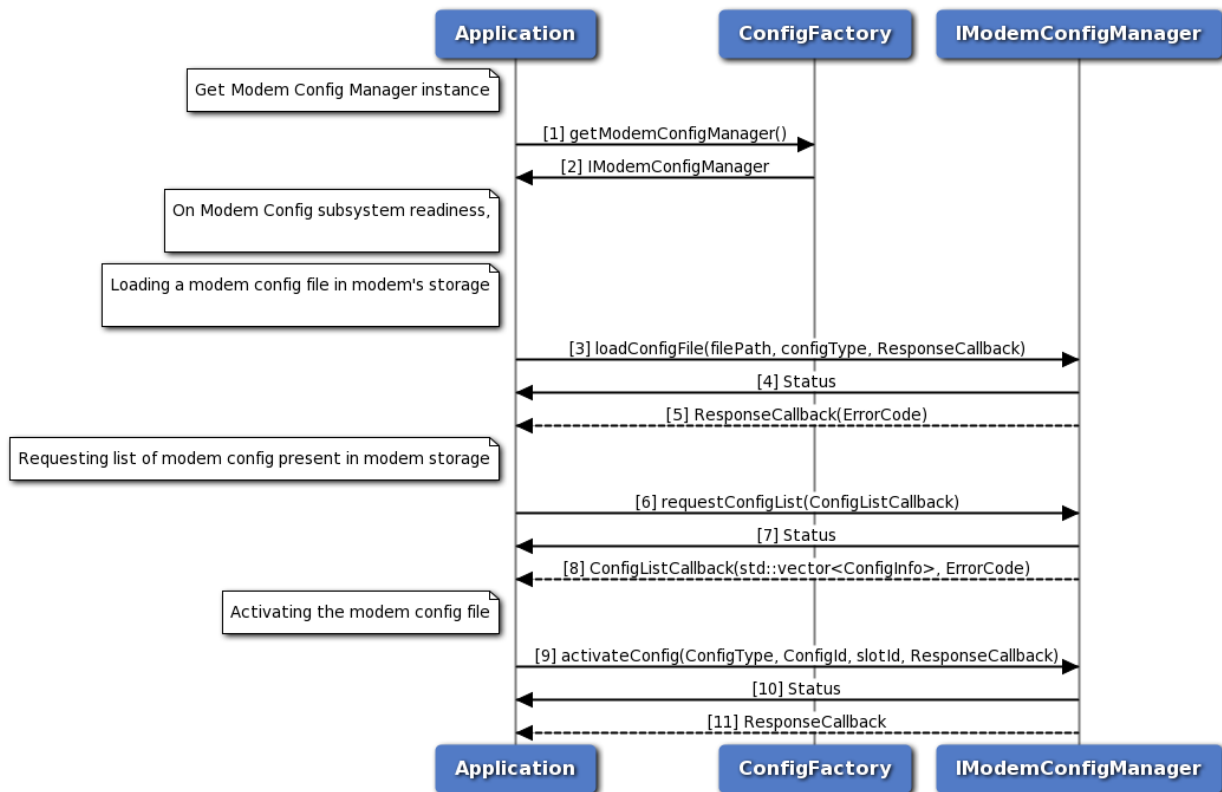
Figure 3-116 Modem Config load and activate call flow
