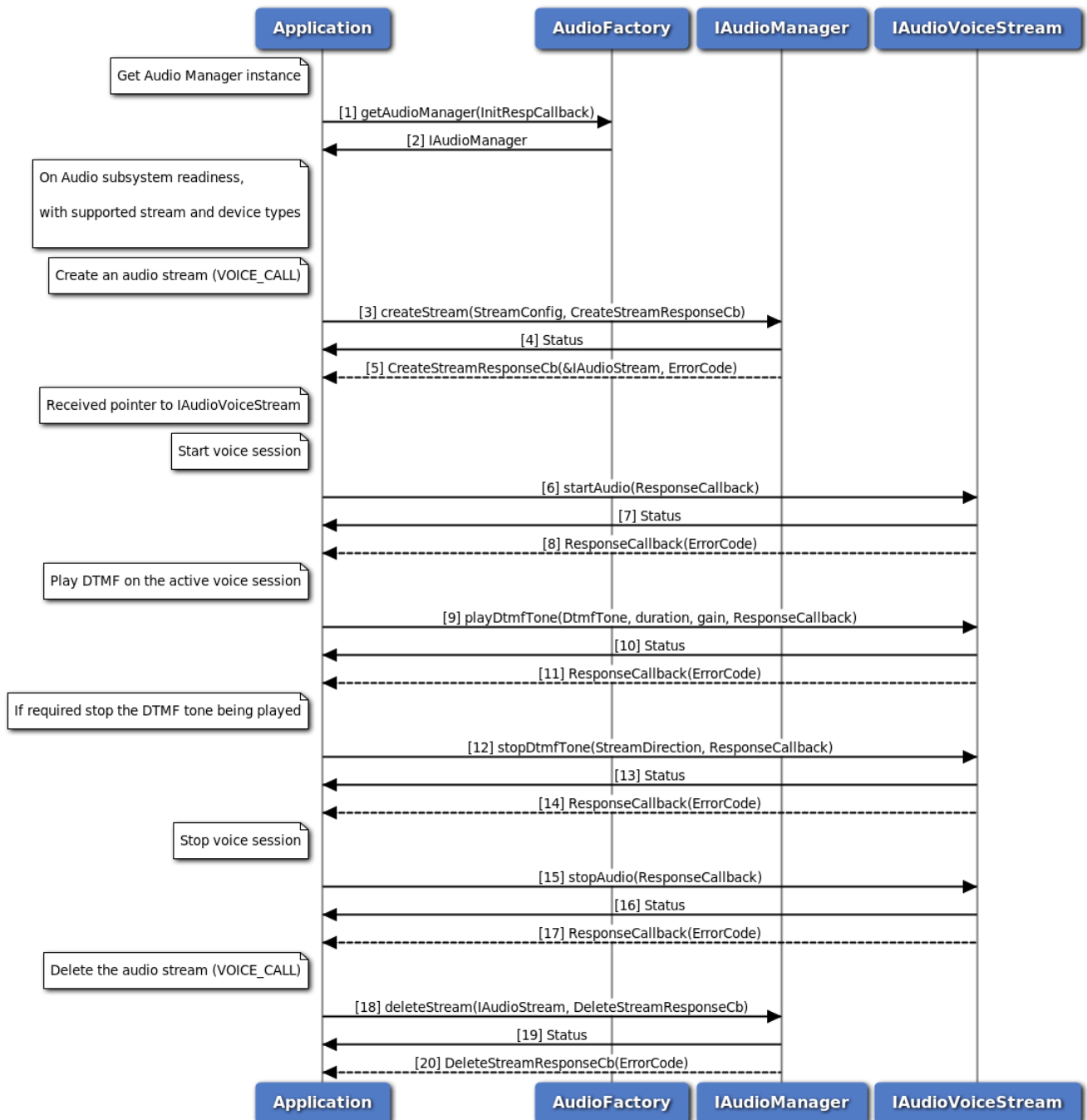
Figure 3-97 Call flow to play DTMF tone
