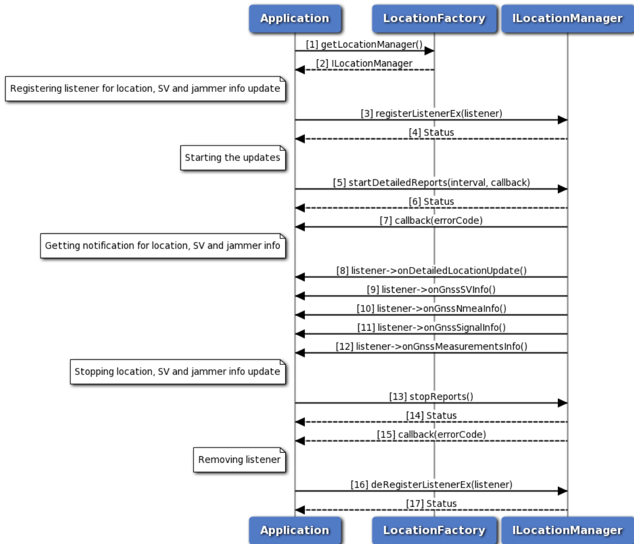
Figure 3-22 Call flow to register/remove listener for generating detailed reports
