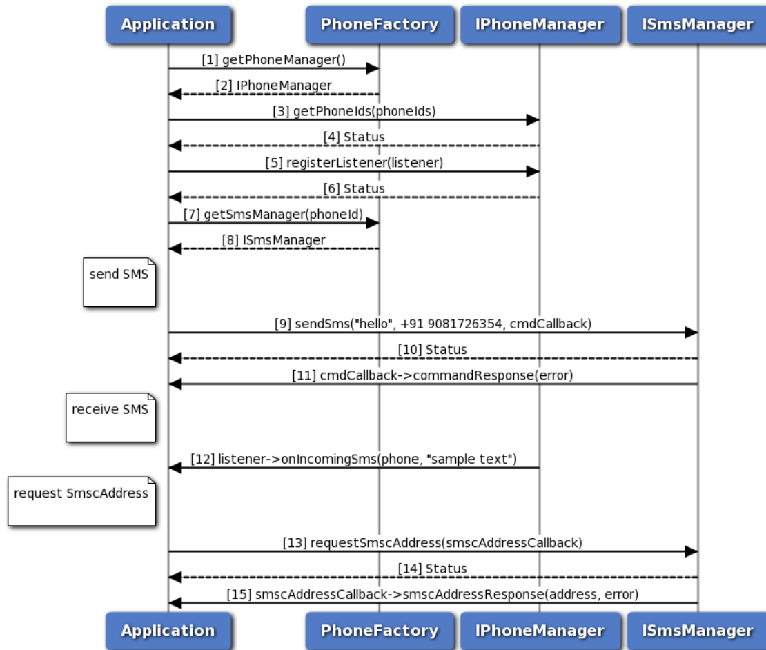
Figure 3-10 SMS call flow
