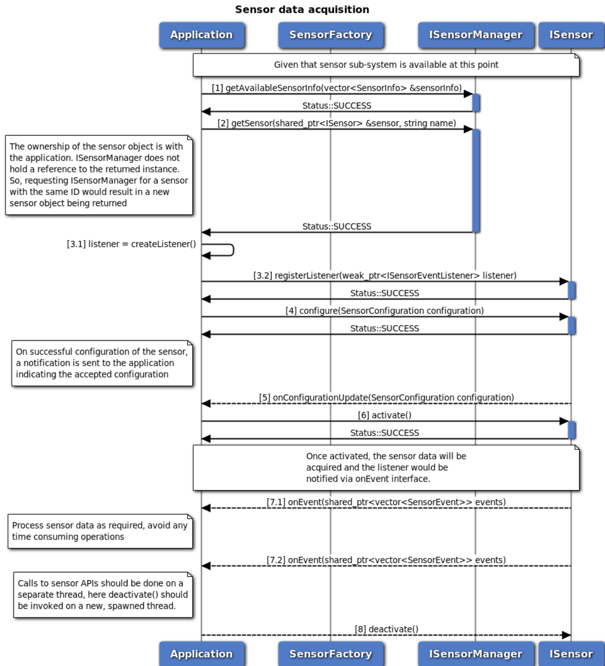
Figure 3-120 Sensor data acquisition call flow
