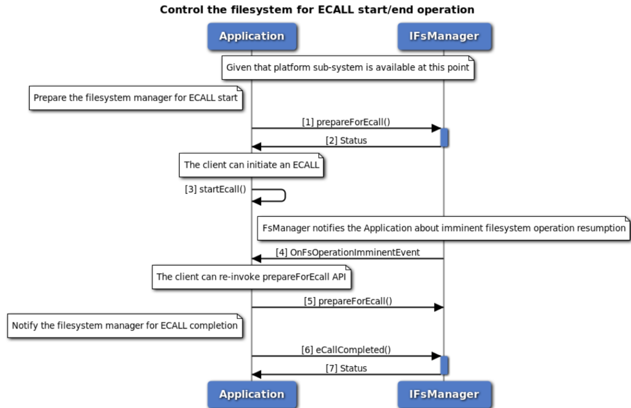
Figure 3-127 Control the filesystem for ECALL operation call flow
