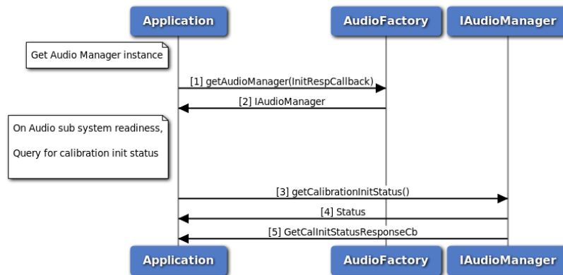
Figure 3-107 Audio calibration configuration status
