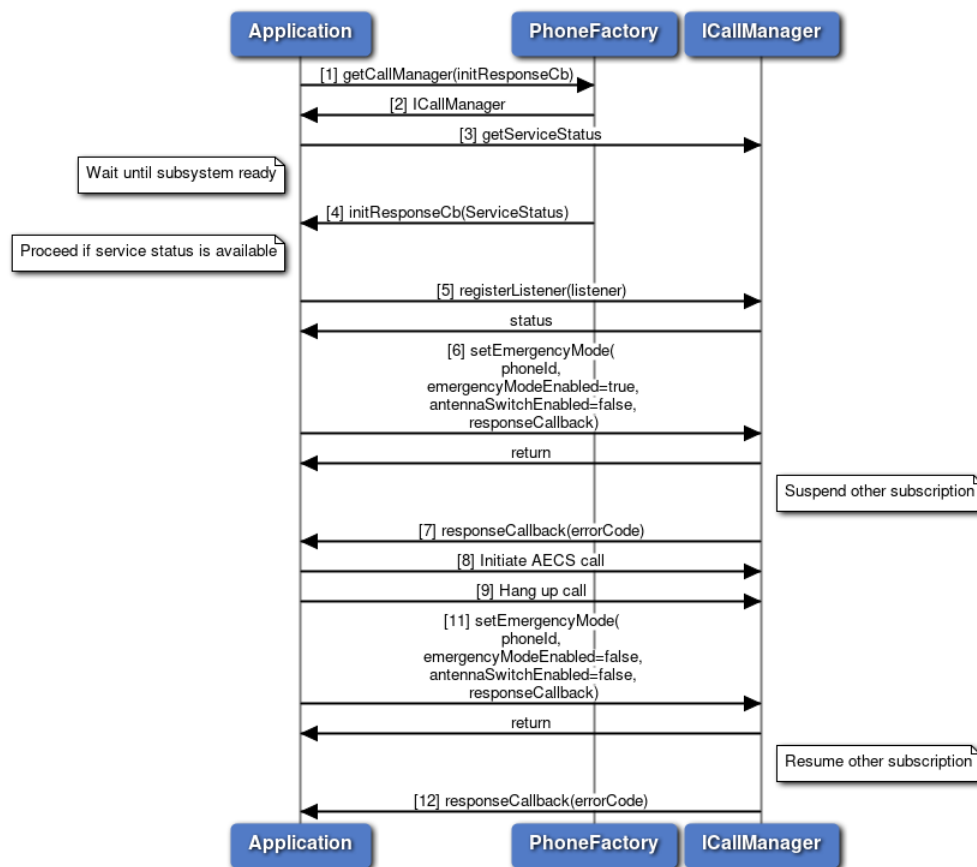
Figure 3-8 Emergency mode call flow
