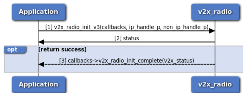
Figure 3-76 C-V2X Radio Initialization Call Flow - C Version
