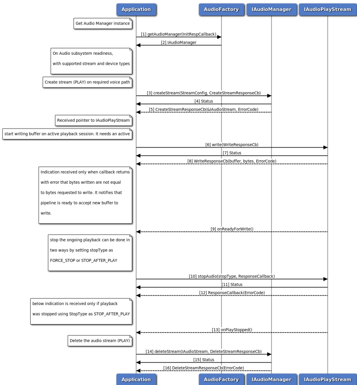
Figure 3-105 Compressed audio format playback on Voice Paths Callflow
