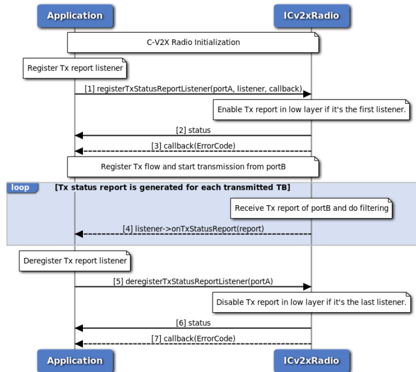
Figure 3-89 C-V2X TX Status Report Call Flow - C++ Version
