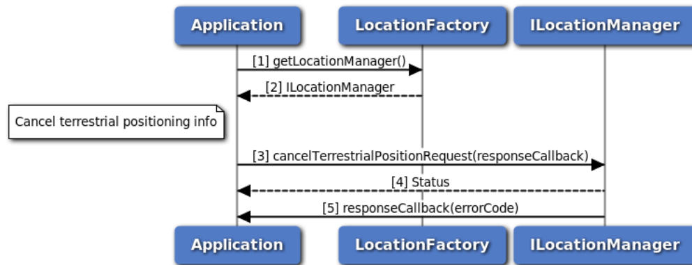
Figure 3-28 Call flow to cancel terrestrial positioning information
