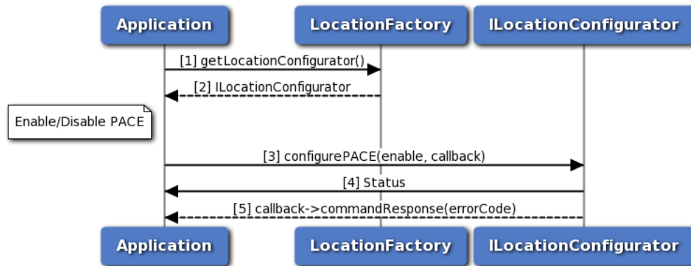
Figure 3-30 Call flow to enable/disable PACE
