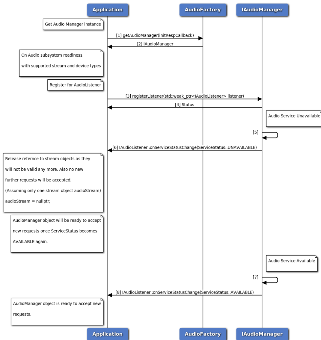
Figure 3-106 Audio Subsystem Restart Callflow
