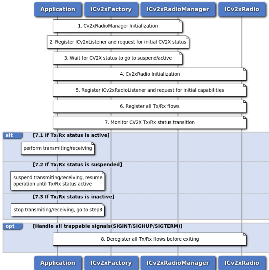
Figure 3-73 C-V2X Radio Control Flow - C++ Version
