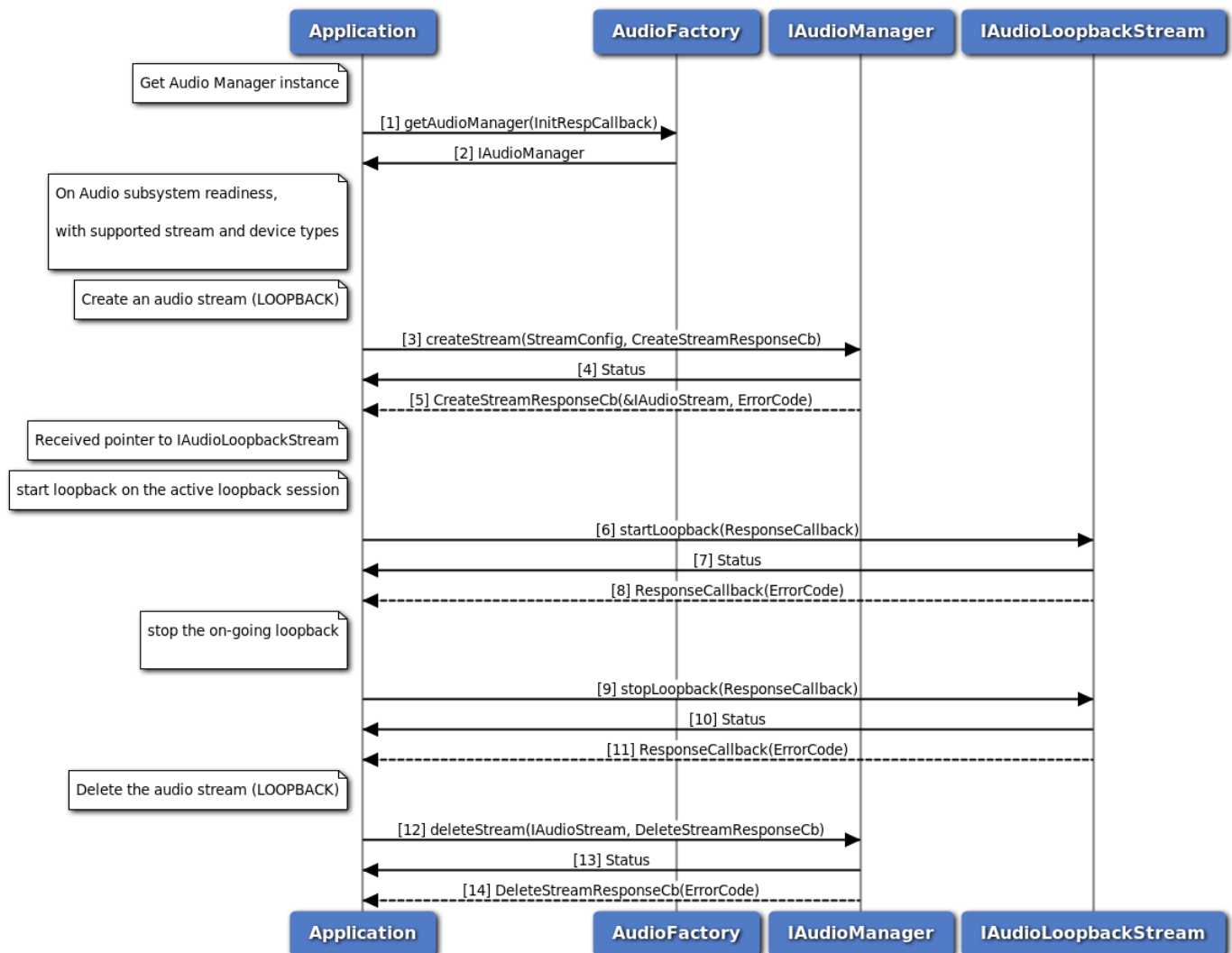
Figure 3-102 Call flow to start/stop loopback between source and sink devices
