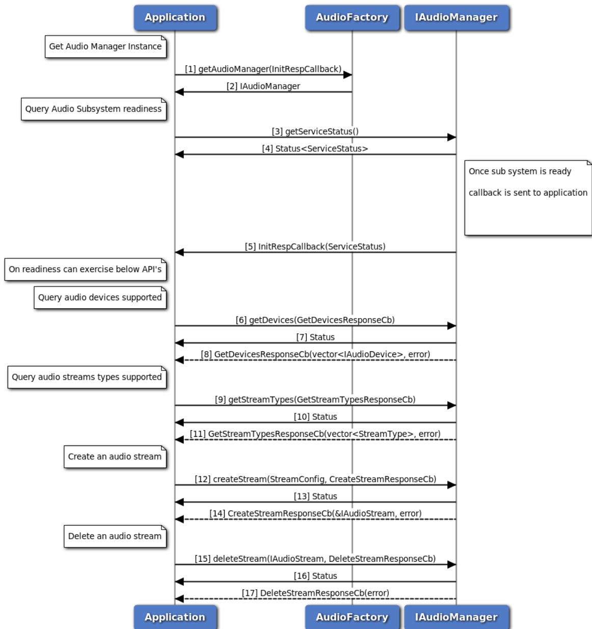
Figure 3-93 Audio Manager API call flow
