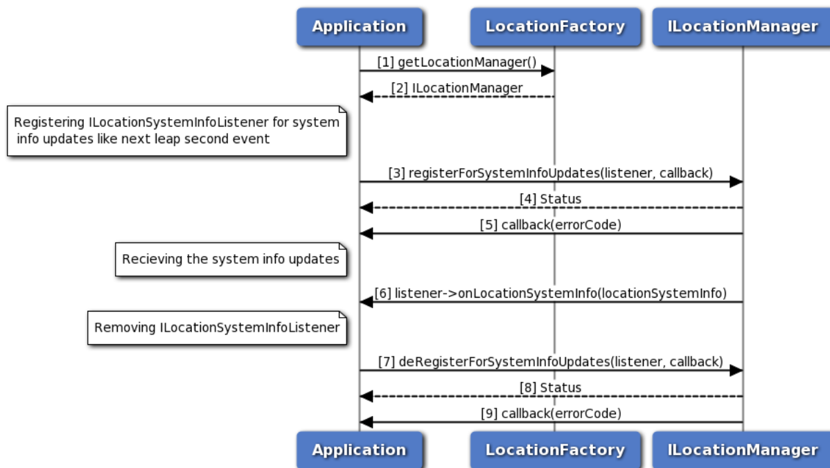
Figure 3-24 Call flow to register/remove listener for system info updates
