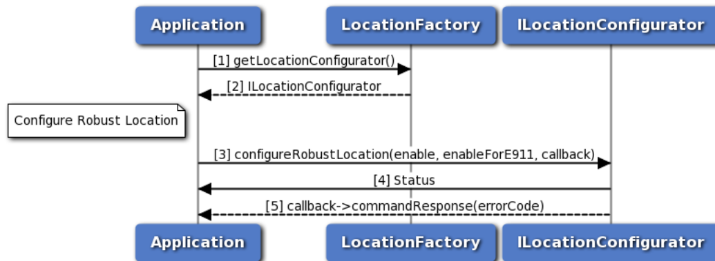
Figure 3-34 Call flow to configure robust location
