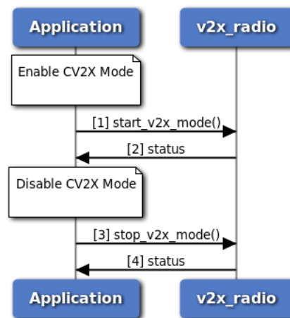
Figure 3-72 Start/Stop C-V2X Mode Call Flow - C Version
