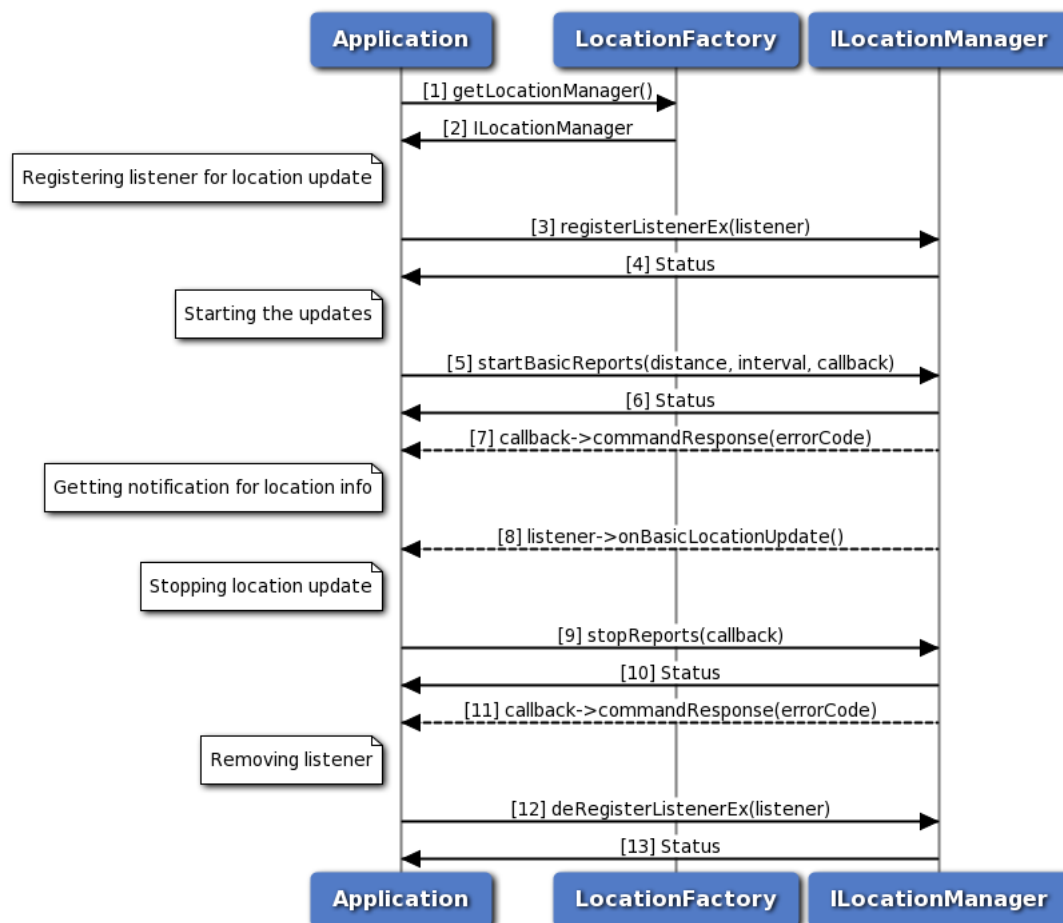
Figure 3-21 Call flow to register/remove listener for generating basic reports
