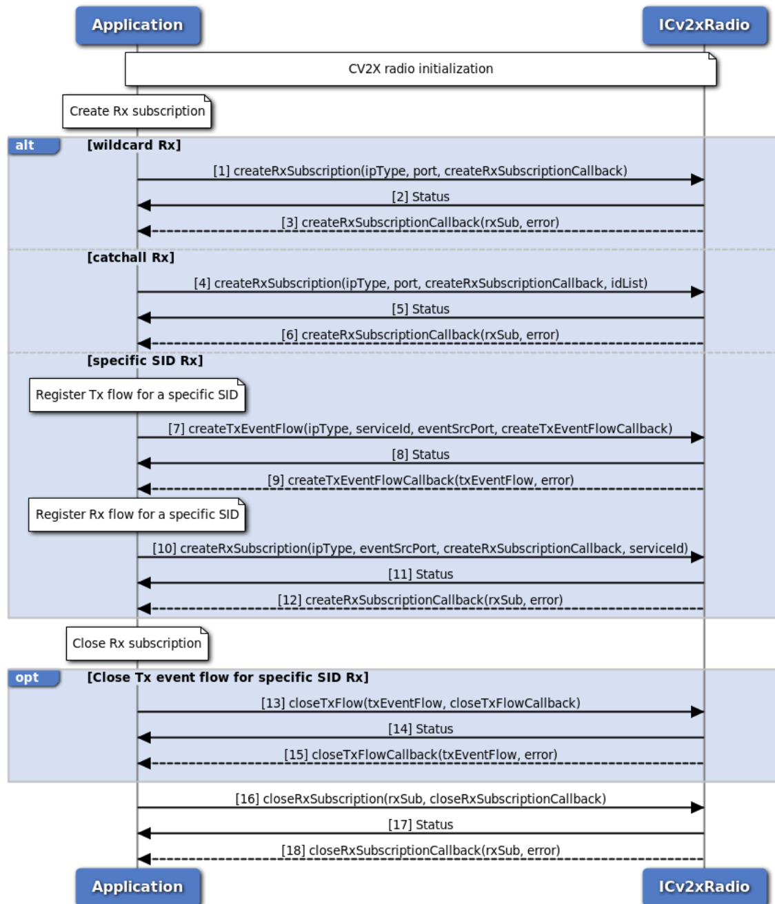
Figure 3-81 C-V2X Radio RX Subscription Call Flow - C++ Version
