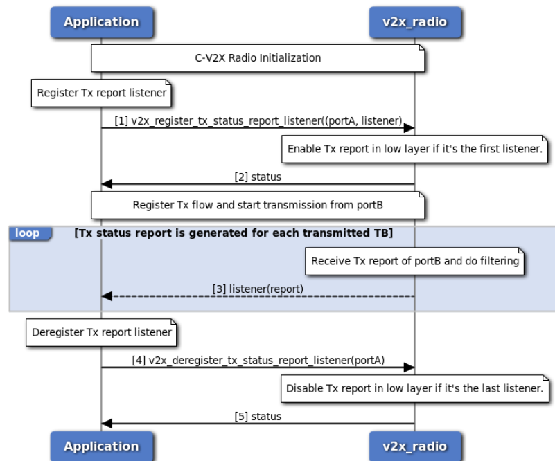
Figure 3-90 C-V2X TX Status Report Call Flow - C Version
