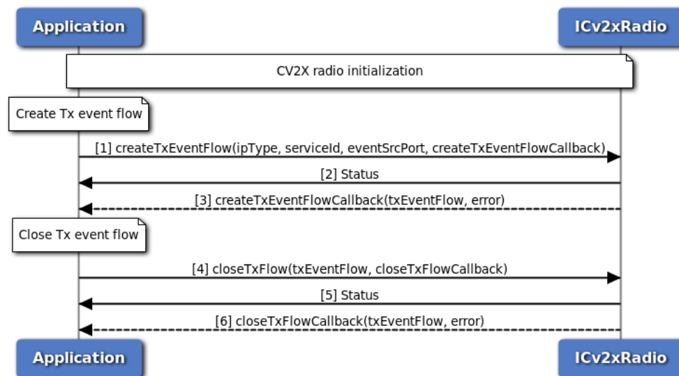
Figure 3-83 C-V2X Radio TX Event Flow Call Flow - C++ Version
