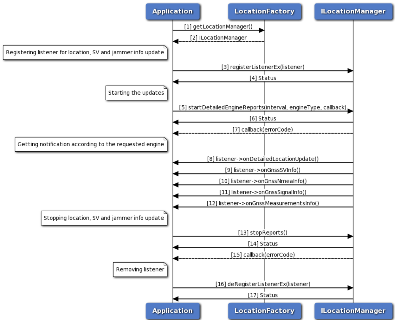
Figure 3-23 Call flow to register/remove listener for generating detailed engine reports
