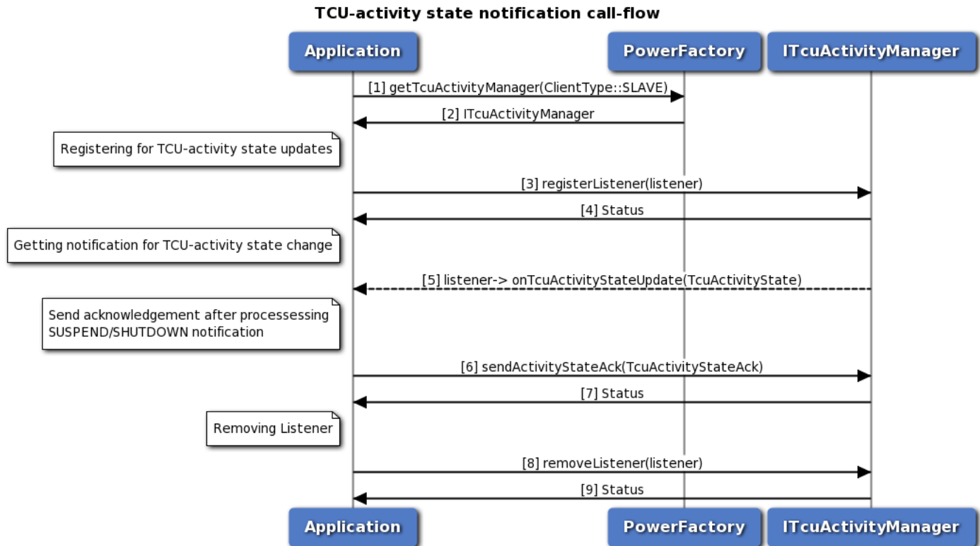
Figure 3-112 Call flow to register/remove listener for TCU-activity manager
