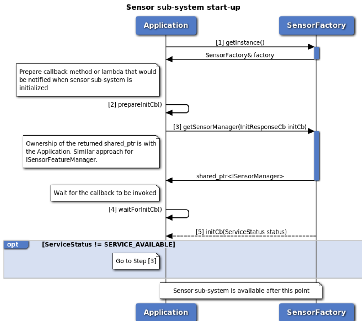
Figure 3-119 Sensor sub-system start-up call flow
