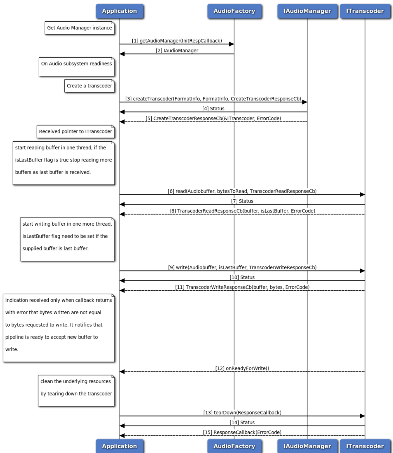
Figure 3-104 Audio Transcoding Operation Callflow
