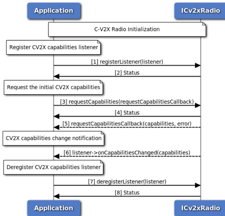
Figure 3-79 Get C-V2X Capabilities Call Flow - C++ Version
