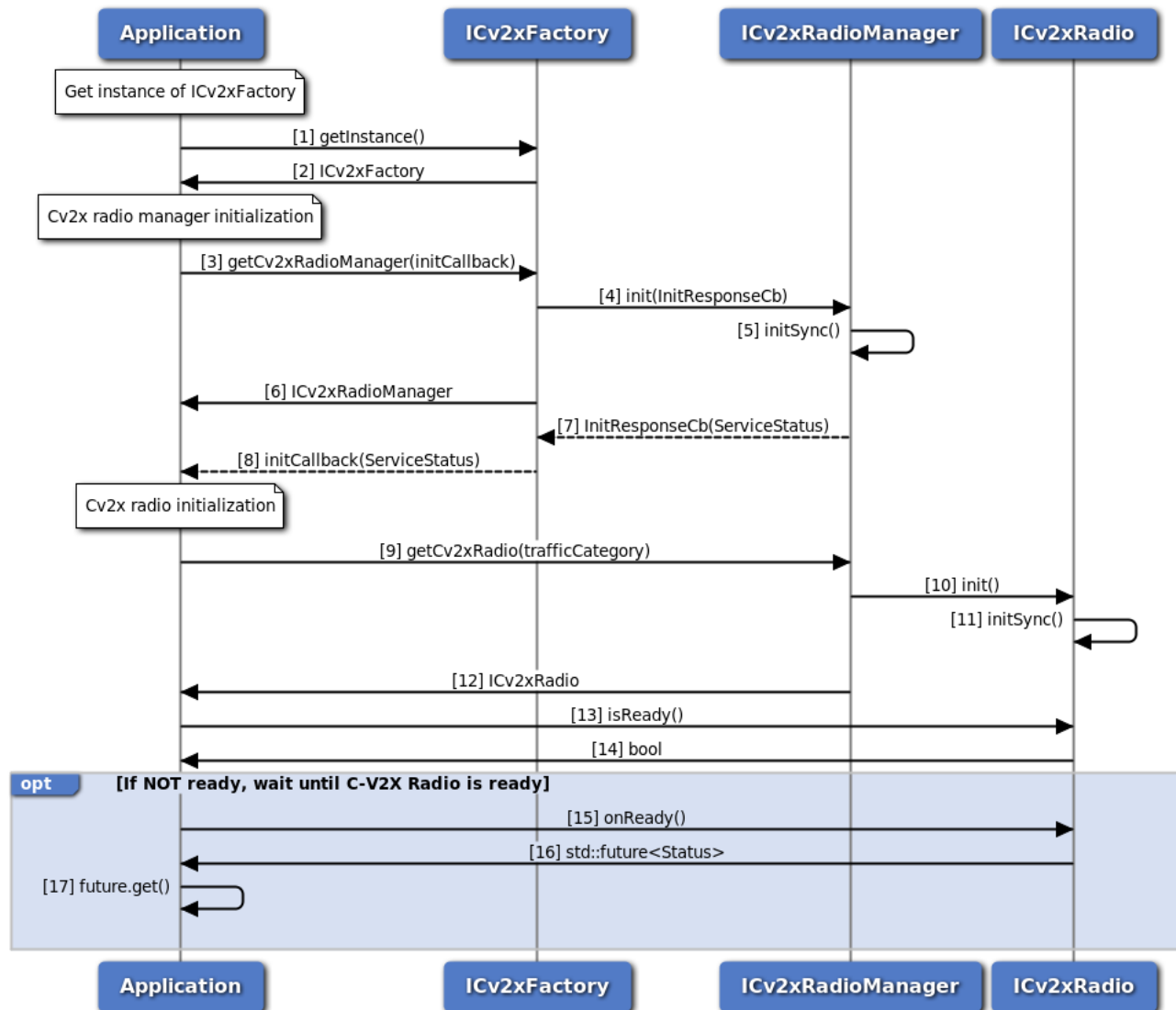
Figure 3-75 C-V2X Radio Initialization Call Flow - C++ Version
