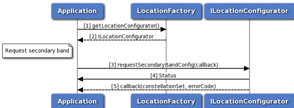
Figure 3-43 Call flow to request secondary band
