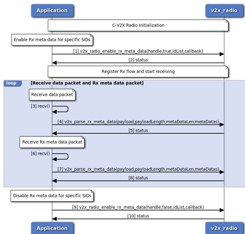
Figure 3-92 C-V2X RX Meta Data Call Flow - C Version
