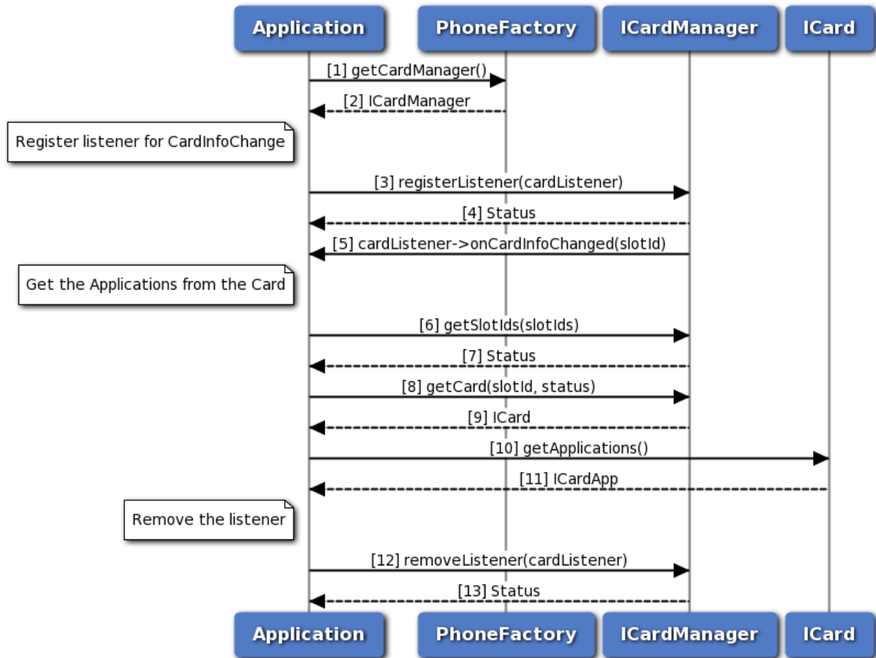
Figure 3-14 Get applications call flow
