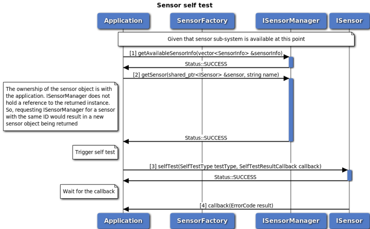
Figure 3-125 Sensor self test call flow
