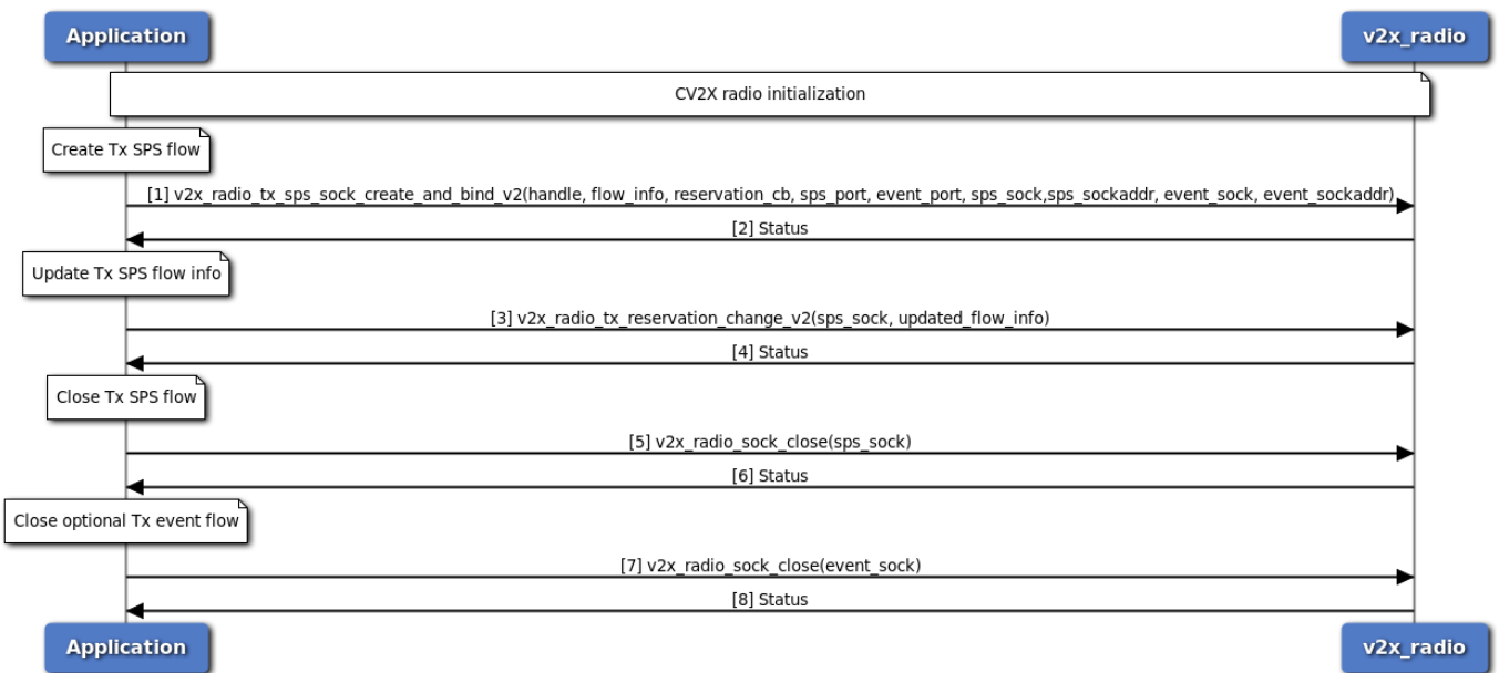
Figure 3-86 C-V2X Radio SPS Flow Call Flow - C Version
