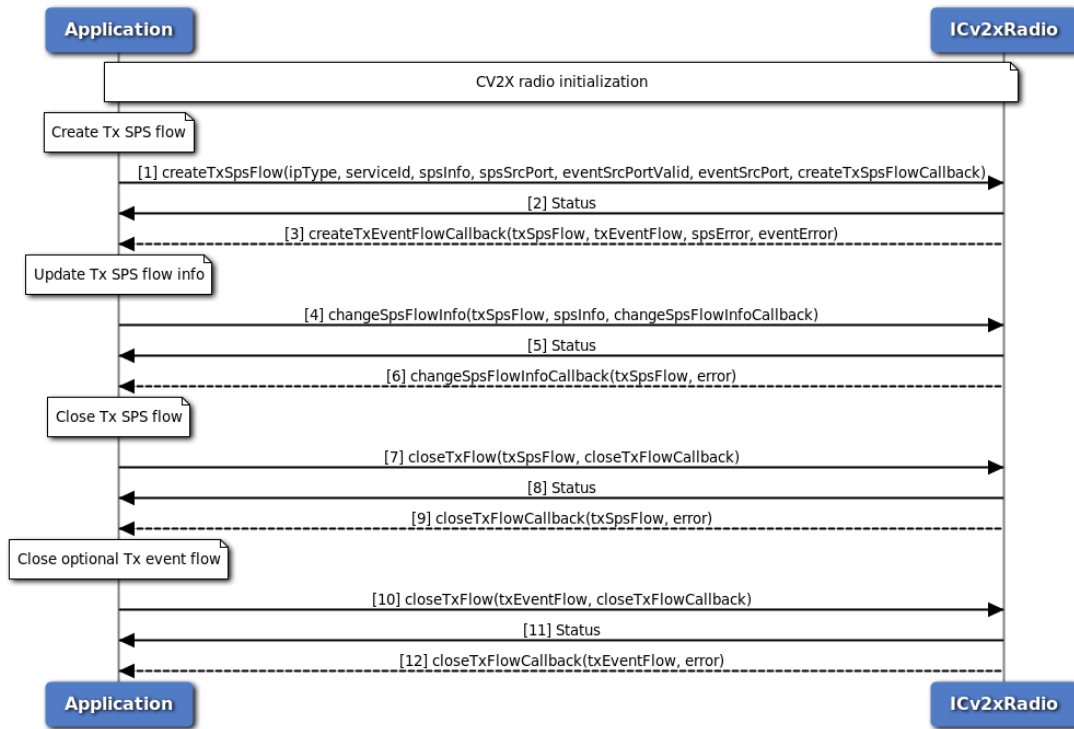
Figure 3-85 C-V2X Radio SPS Flow Call Flow - C++ Version
