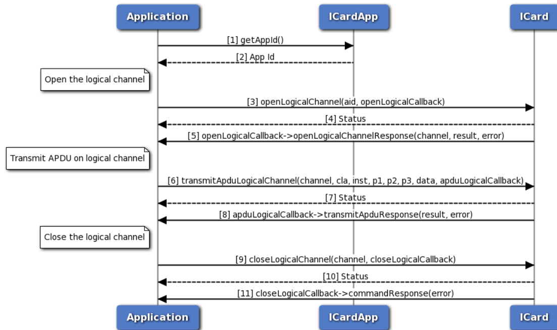
Figure 3-15 On logical channel
