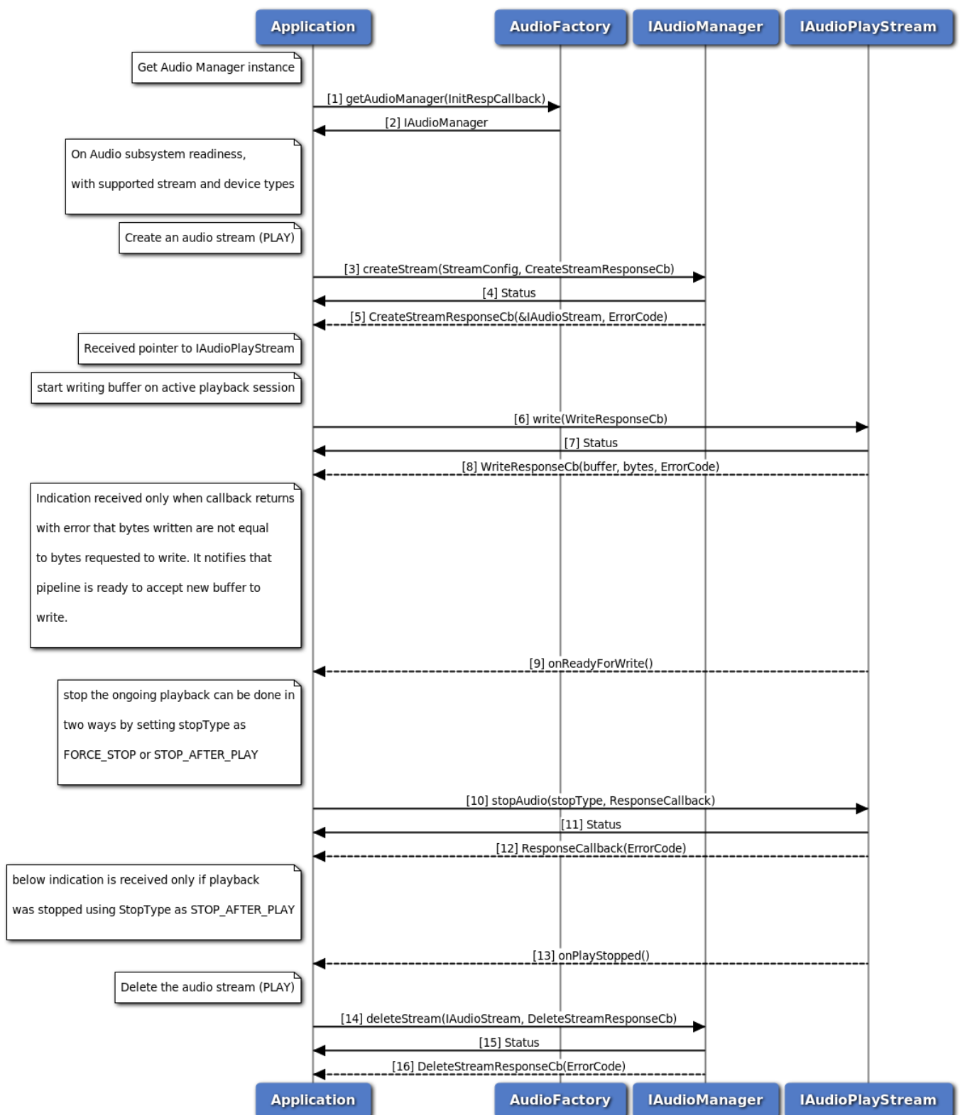
Figure 3-103 Call flow to play Compressed audio format
