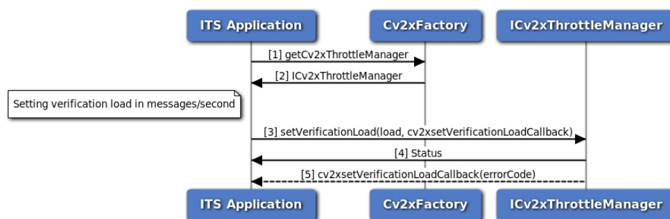
Figure 3-88 C-V2X Throttle Manager set verification call flow
