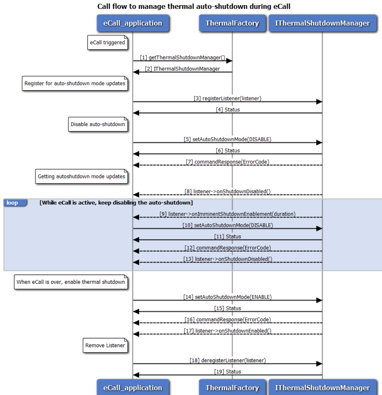
Figure 3-111 Call flow to manage thermal auto-shutdown from an eCall application
