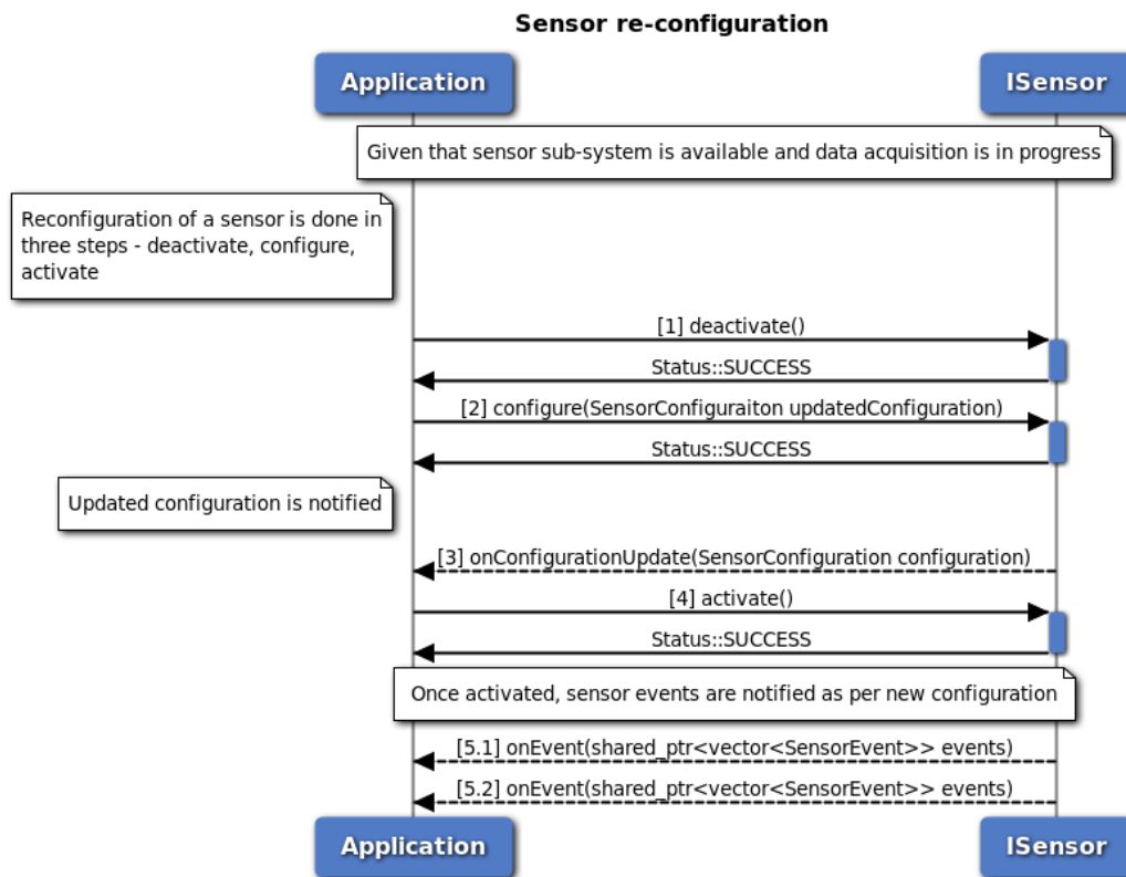
Figure 3-121 Sensor reconfiguration call flow
