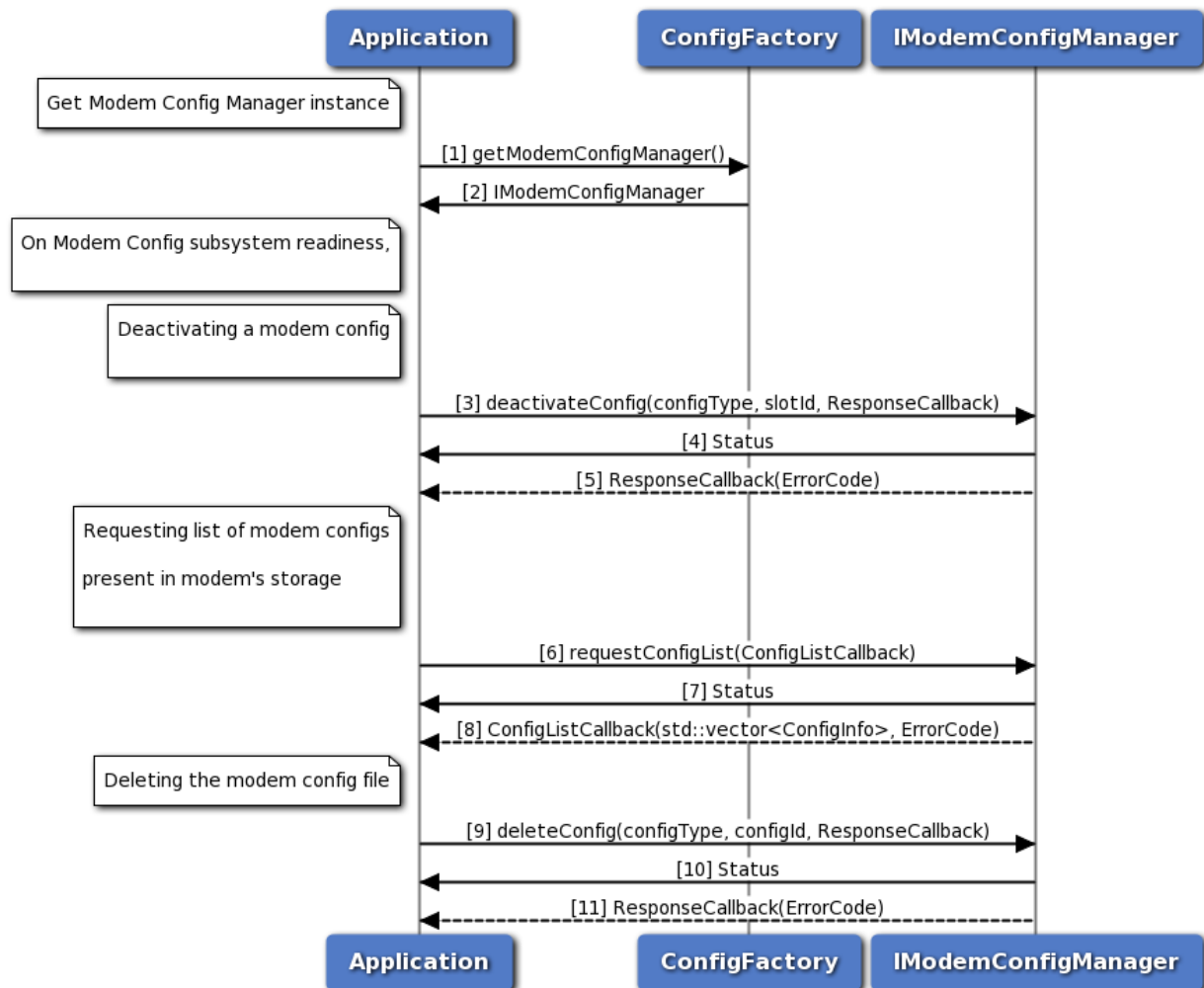
Figure 3-117 Modem Config deactivate and delete Call Flow
