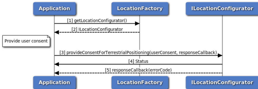
Figure 3-45 Call flow to provide user consent for terrestrial positioning
