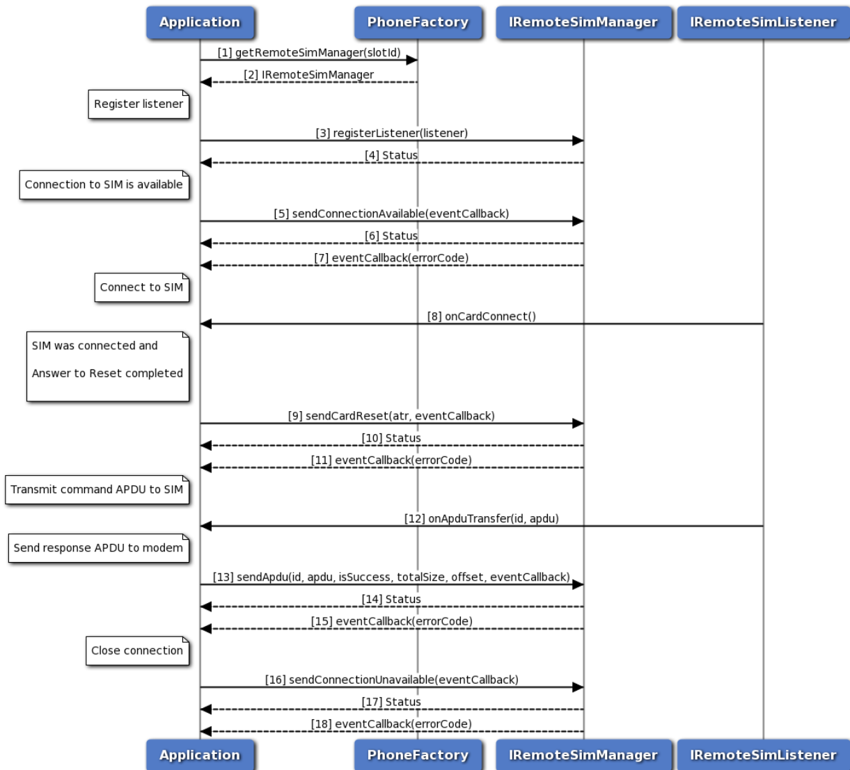
Figure 3-115 Remote SIM call flow
