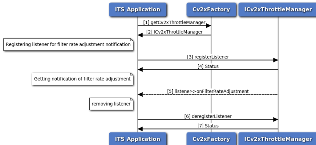
Figure 3-85 C-V2X Throttle Manager Filter Rate Adjustment Notification call flow
