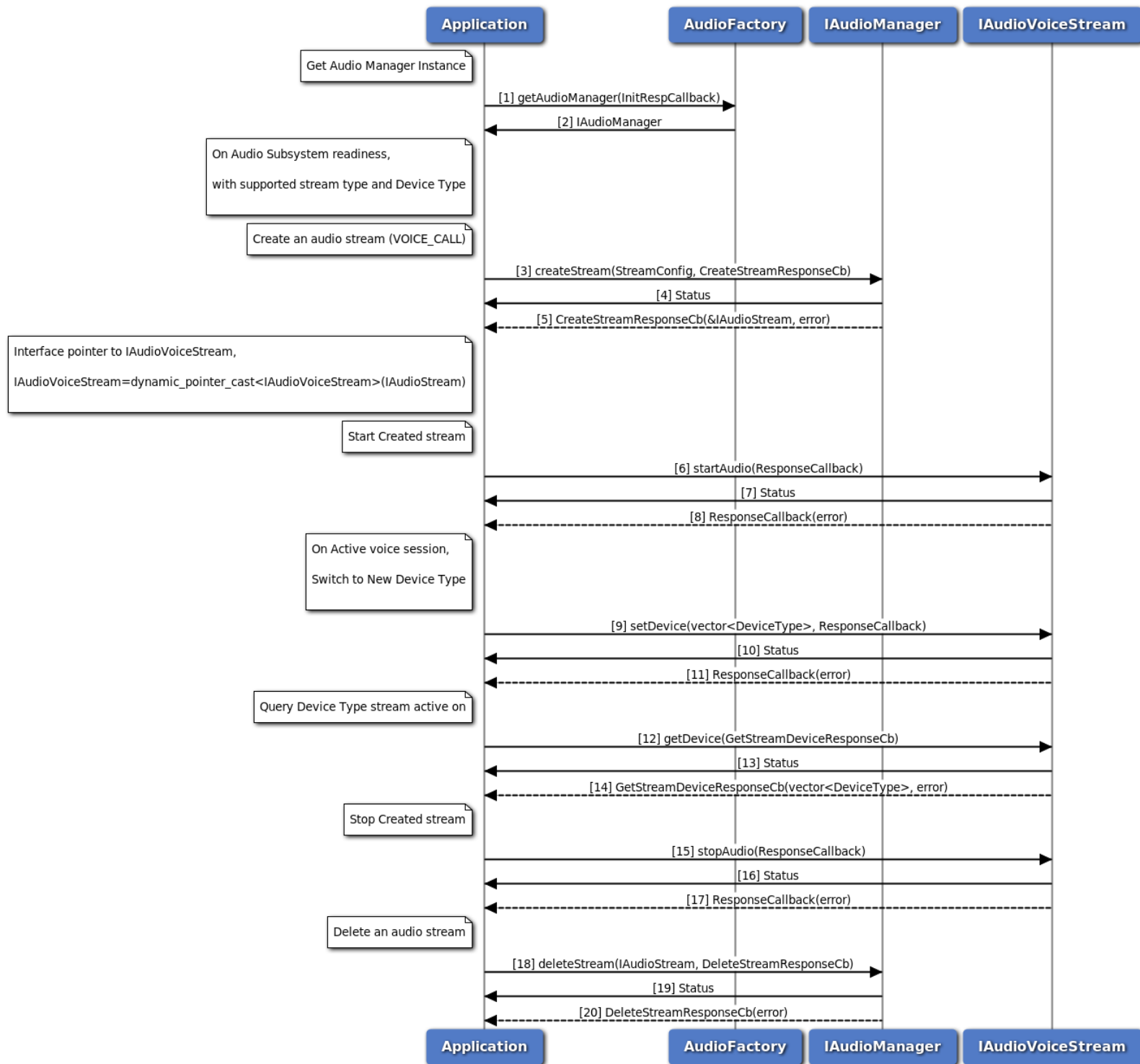
Figure 3-93 Audio Voice Call Device Switch call flow
