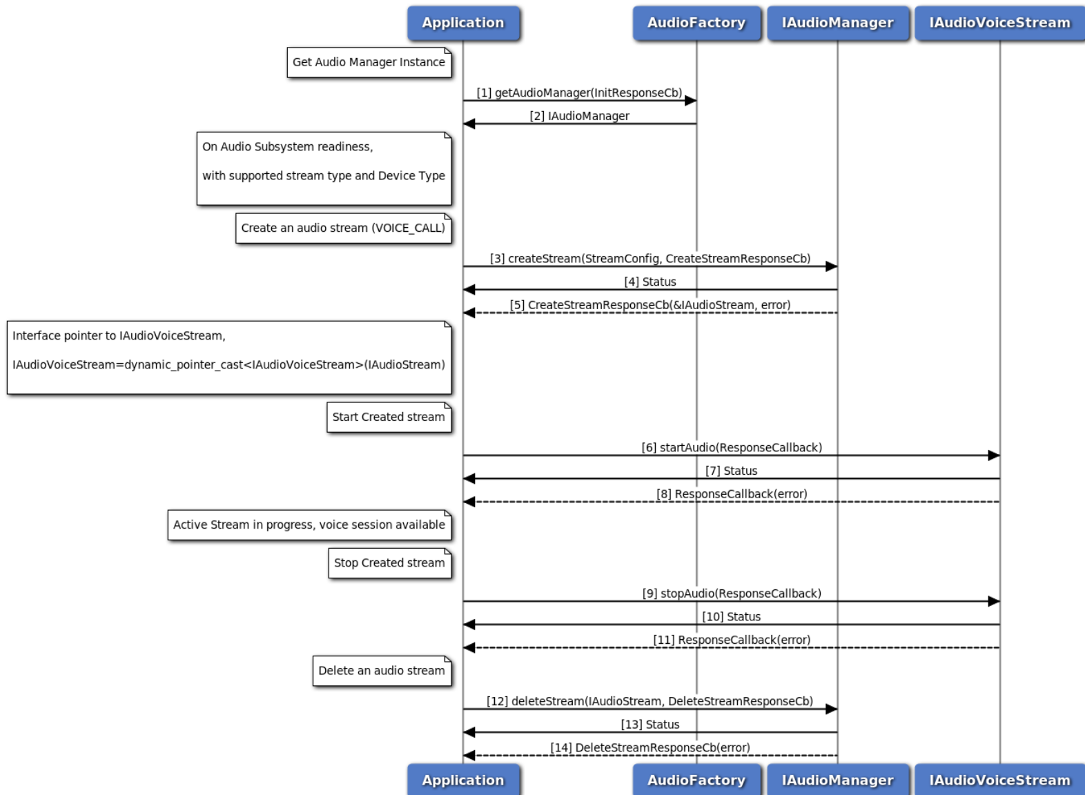
Figure 3-92 Audio Voice Call Start/Stop call flow
