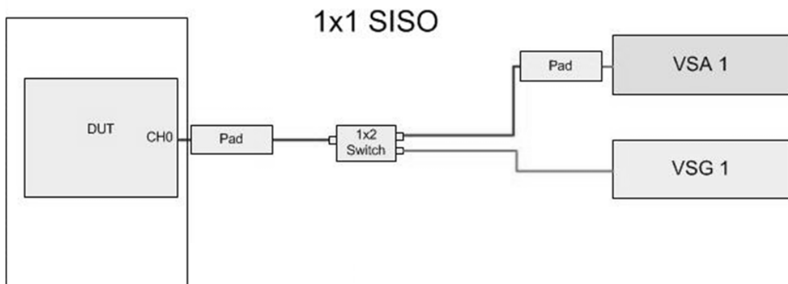
Figure 1-1 DVT test setup for Wi-Fi testing
